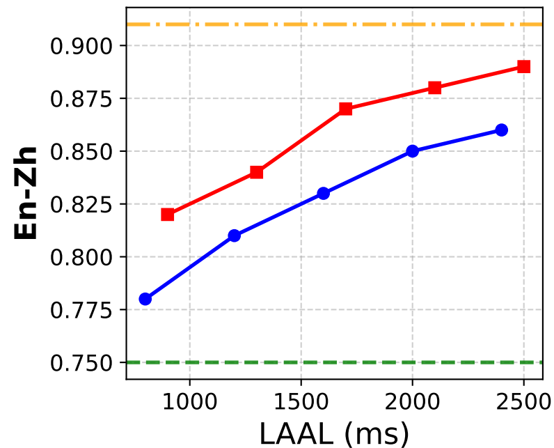
COMET
