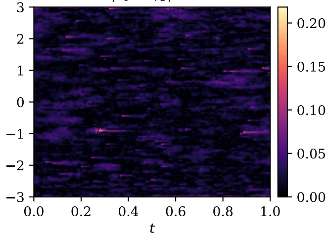
volatility y(x, t) \max |u_\theta - u_{\text{FD}}| = 0.218
