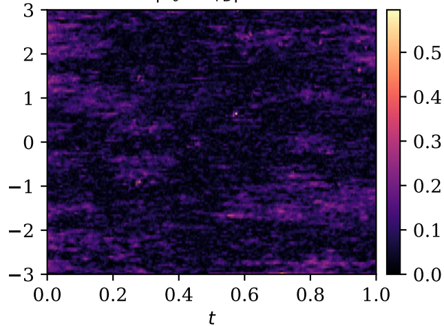
price z(x, t) \max |u_\theta - u_{\text{FD}}| = 0.596
