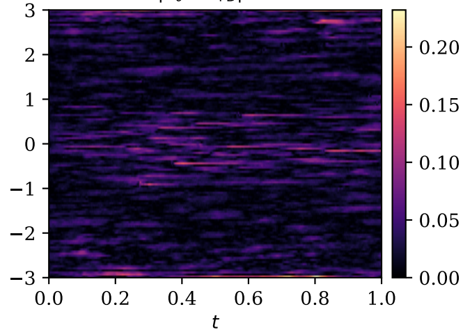
jump intensity p(x, t) \max |u_\theta - u_{\text{FD}}| = 0.232
