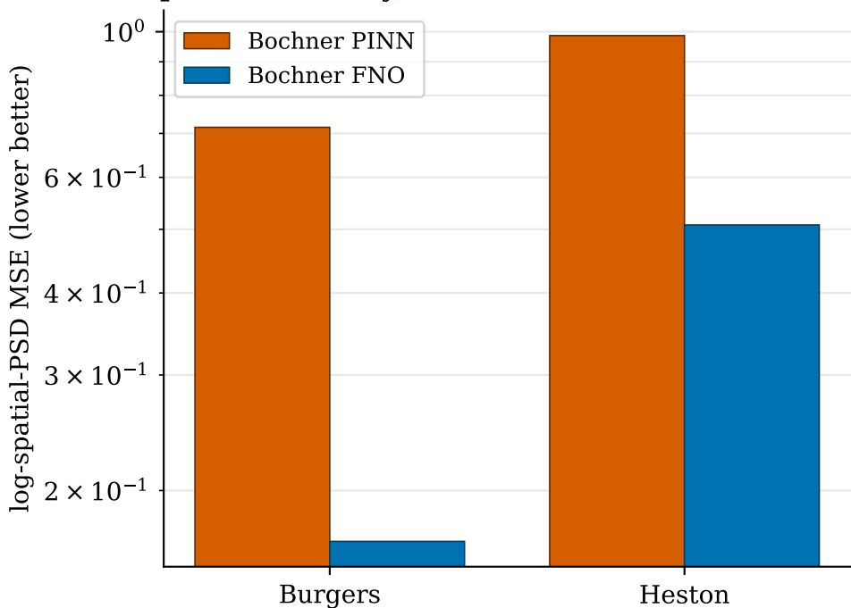
Spectrum fidelity, Bochner PINN vs Bochner FNO
