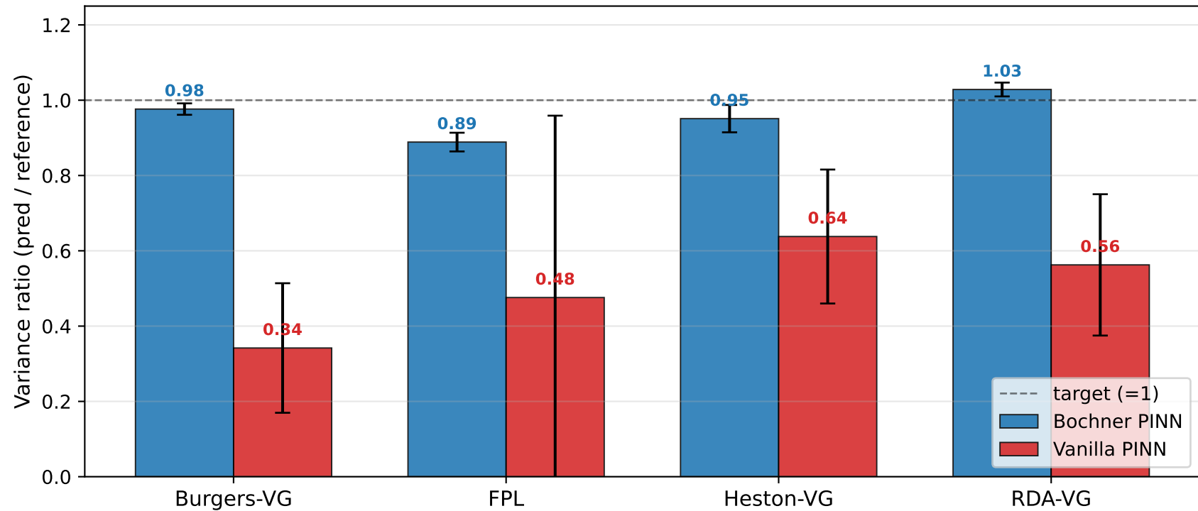
3D generalisation: variance-gap closure across four SPDE families
