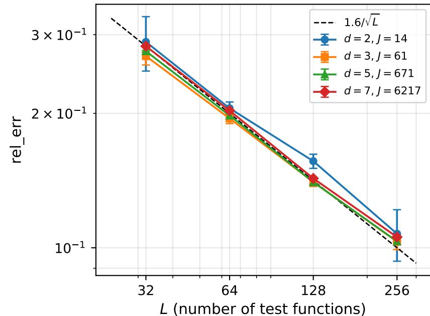
(a) Half-period basis: uniform-in- d
