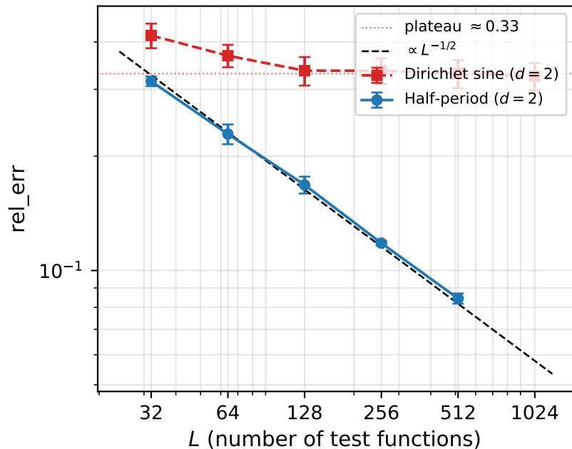
(b) Dirichlet sine plateau vs half-period
