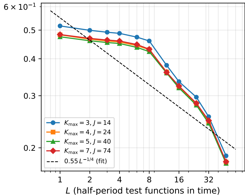
(a) ERA5 2m temperature, 90 d \times 16 \times 16 grid: uniform in K_{\max}
