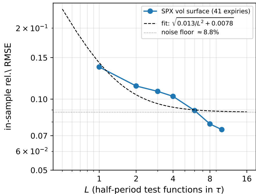
(b) SPX implied vol surface, K_{\max} = 4 : noise-floor saturation
