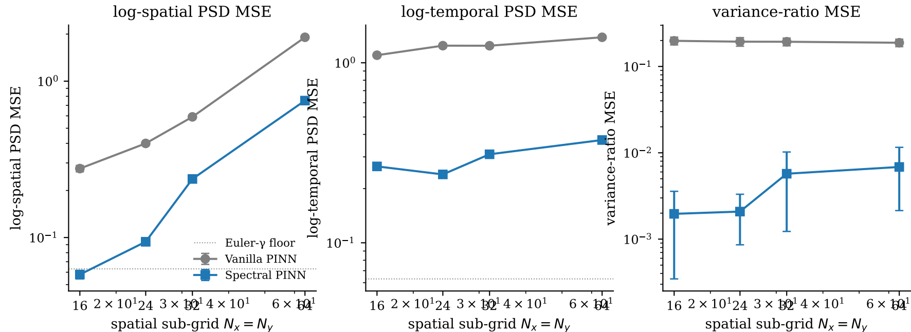
Grid convergence on Burgers-VG (5 validation seeds)
