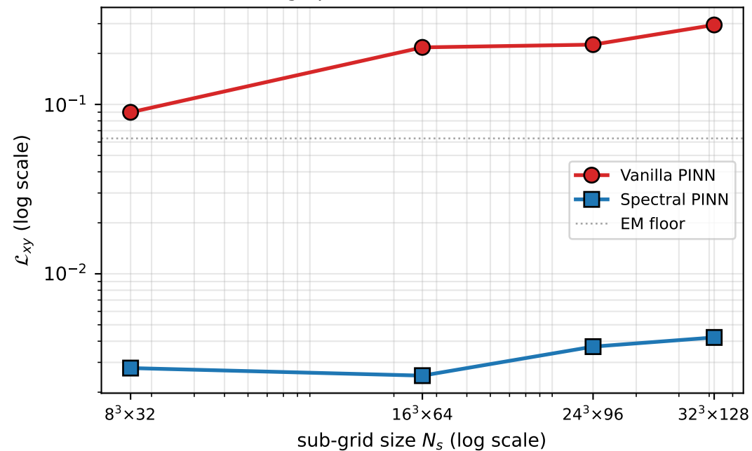
(a) Log-spatial PSD MSE vs. resolution
