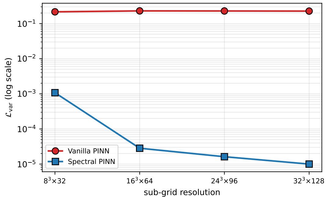
(b) Variance loss vs. resolution
