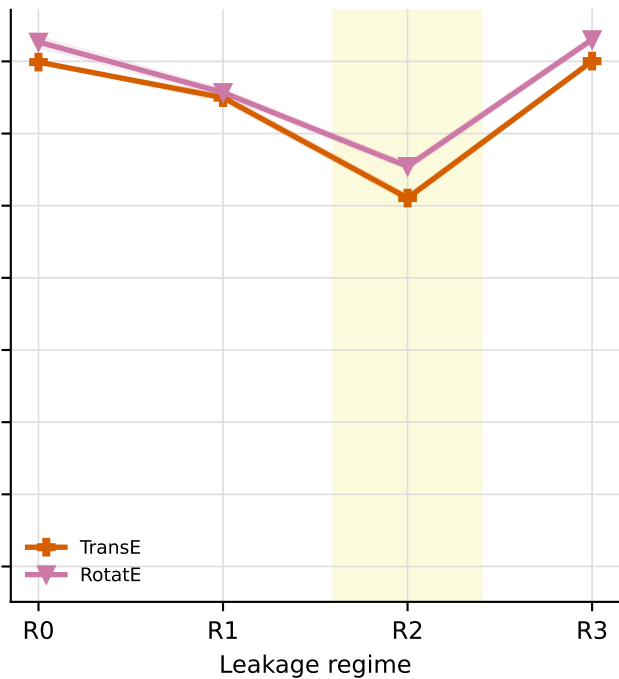
KGE models
