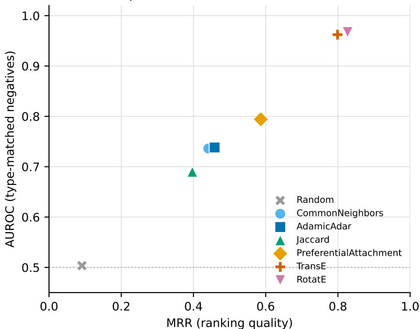
AUROC compresses the differences MRR reveals (R0)
