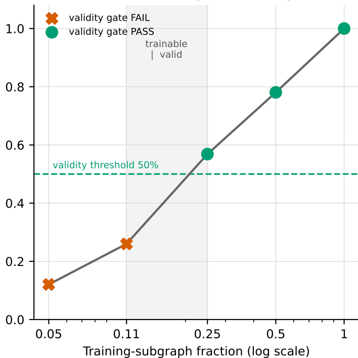
The leak dissolves with the subsample — and returns only out of budget
