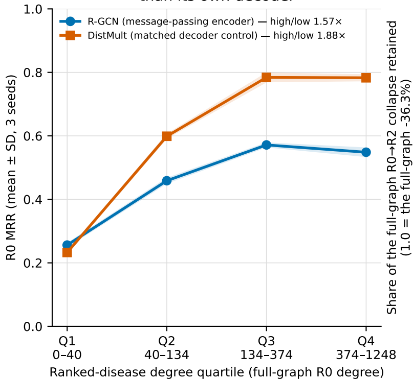
Message passing rides target popularity less than its own decoder
