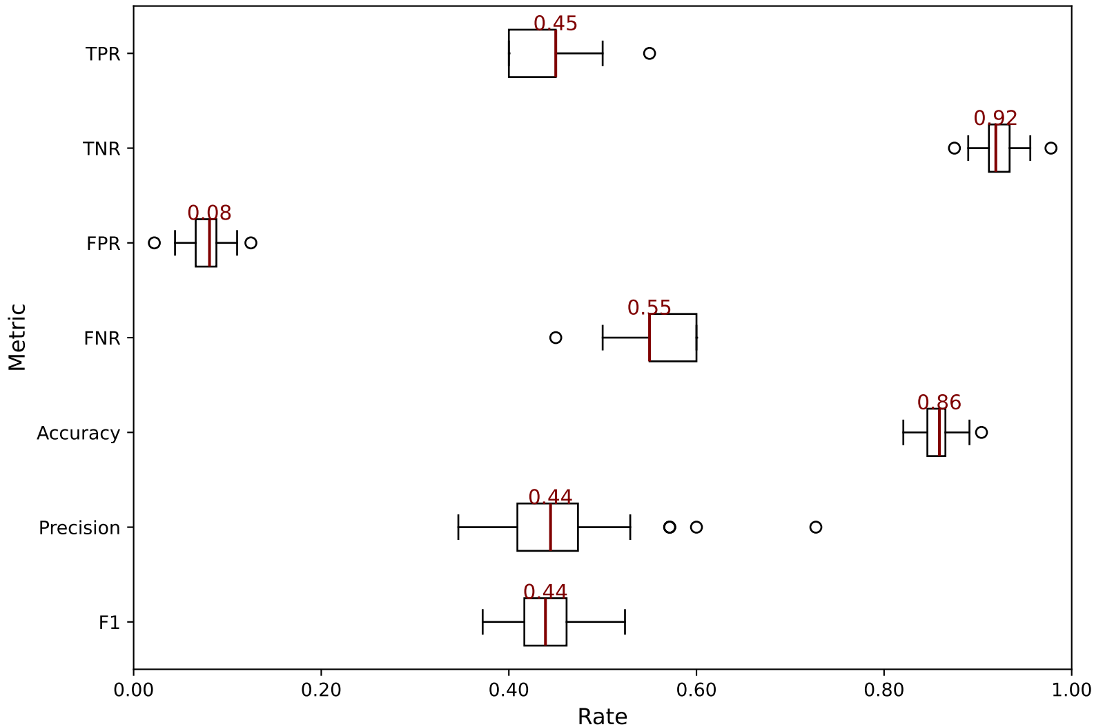
PM / M1: Detection Rate Distribution (100 runs)
