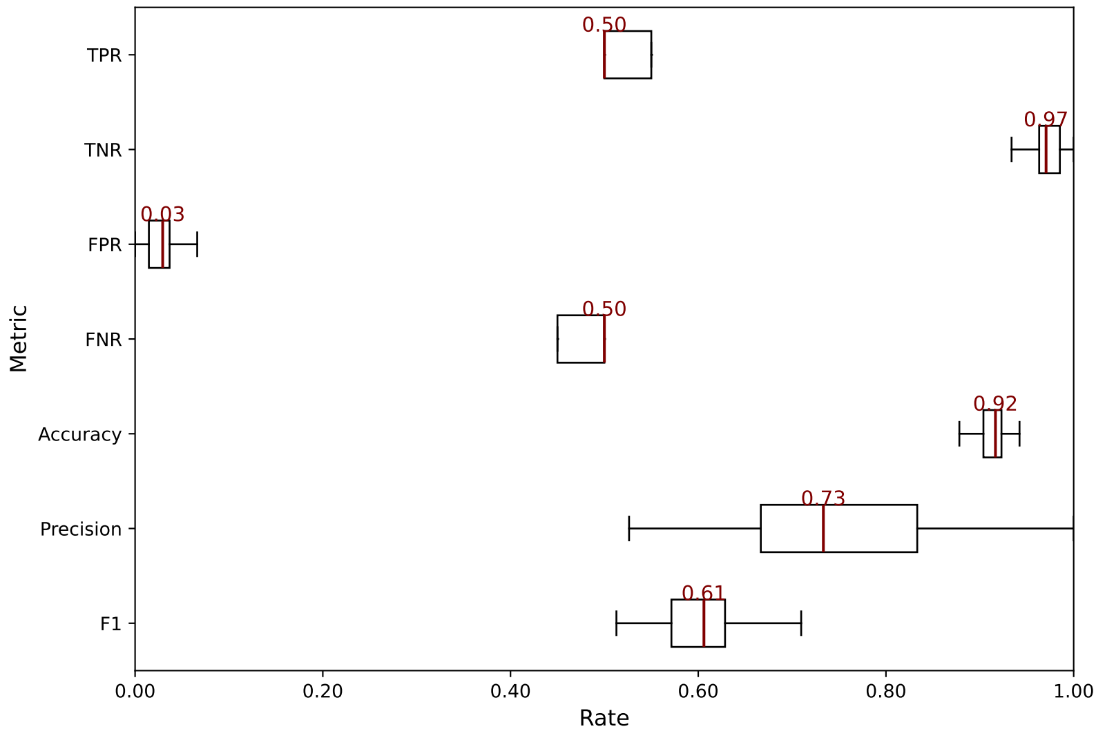
PM / M2: Detection Rate Distribution (100 runs)
