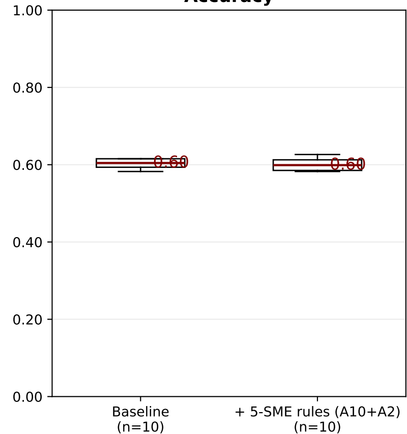
Accuracy
