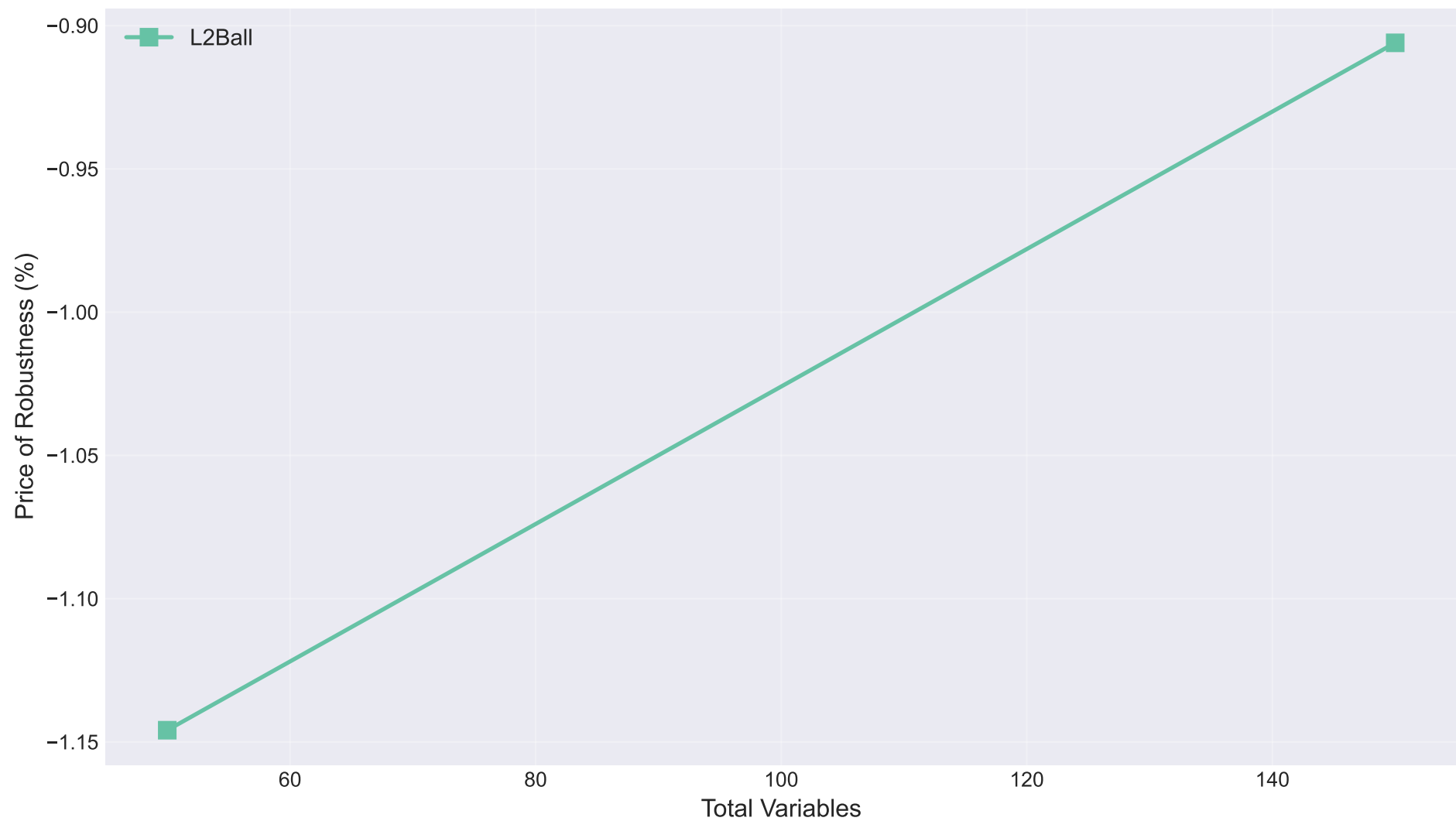
Price of Robustness vs Problem Size
