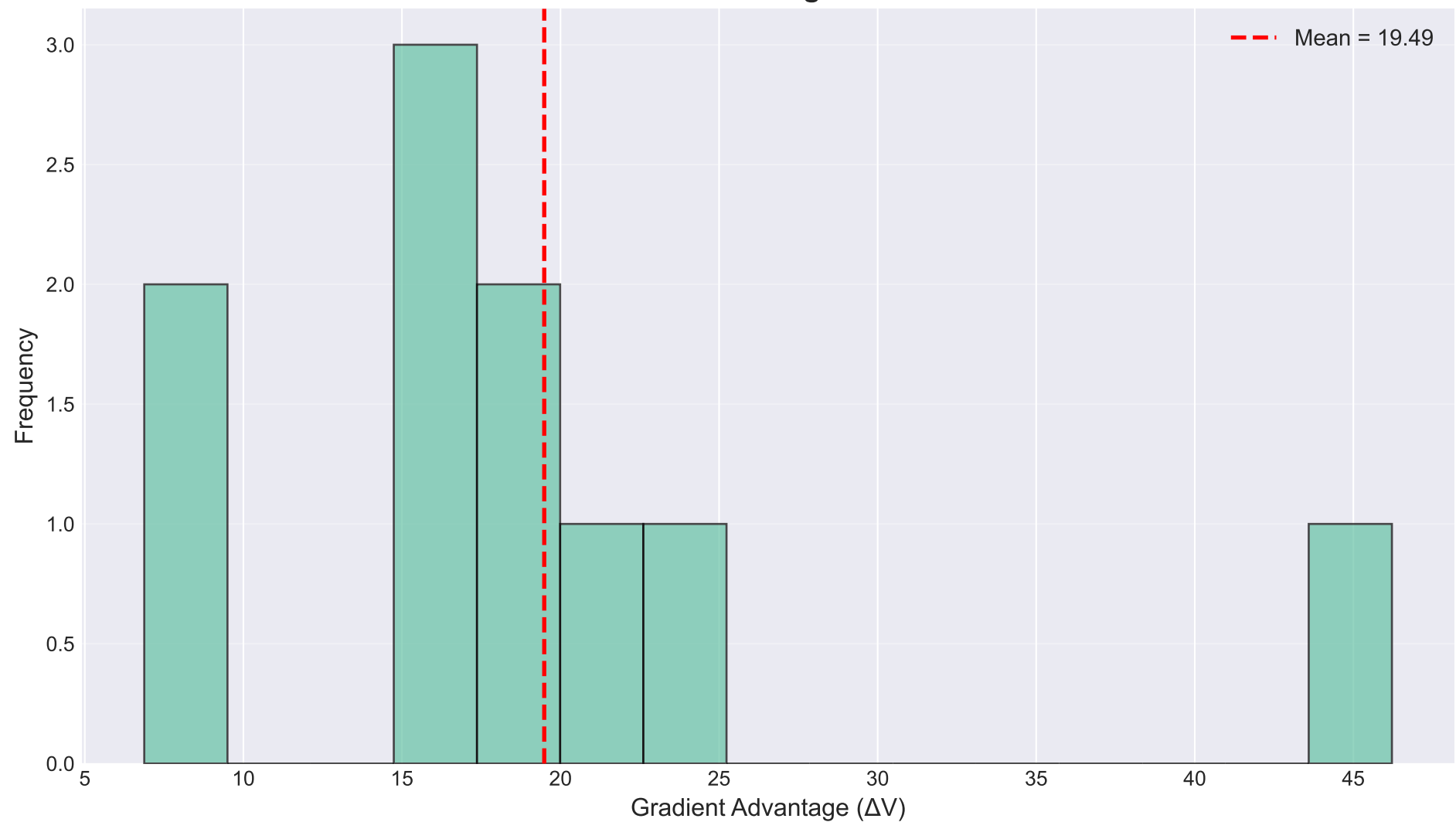
Distribution of Gradient Advantage over Random Directions
