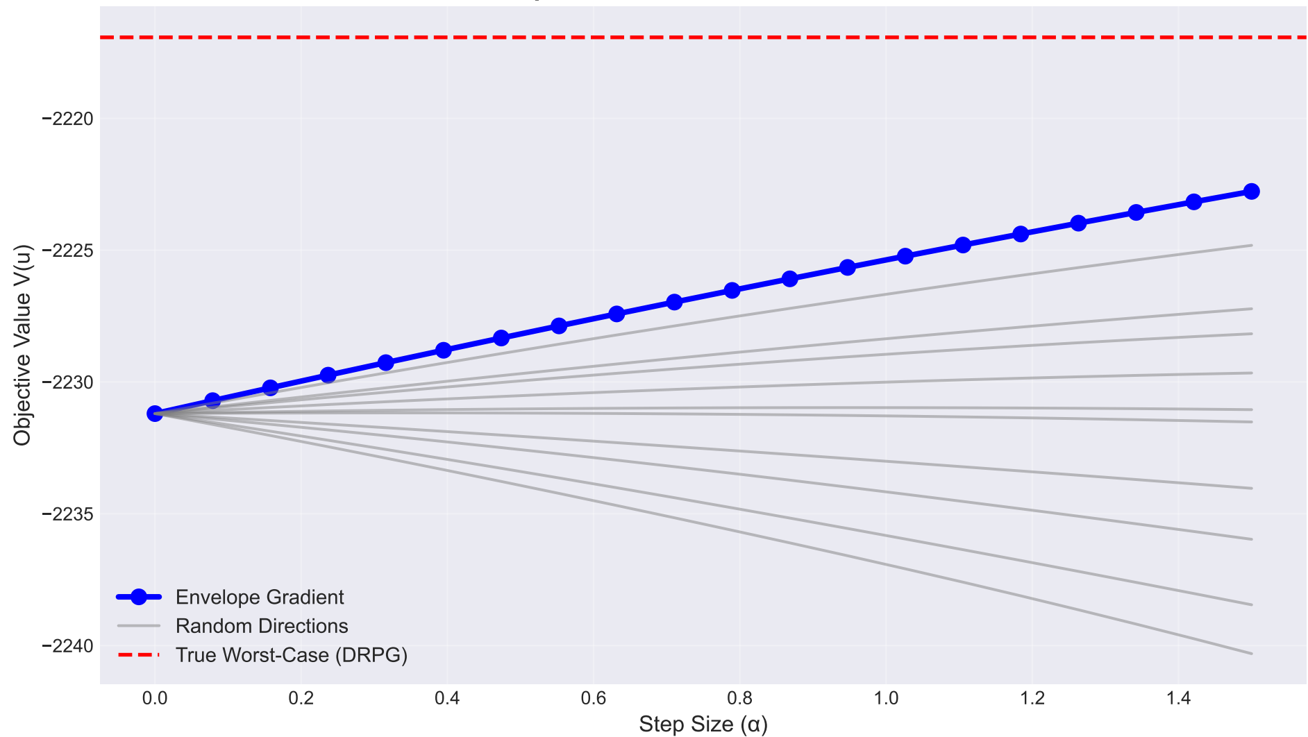
Envelope Gradient vs Random Directions
