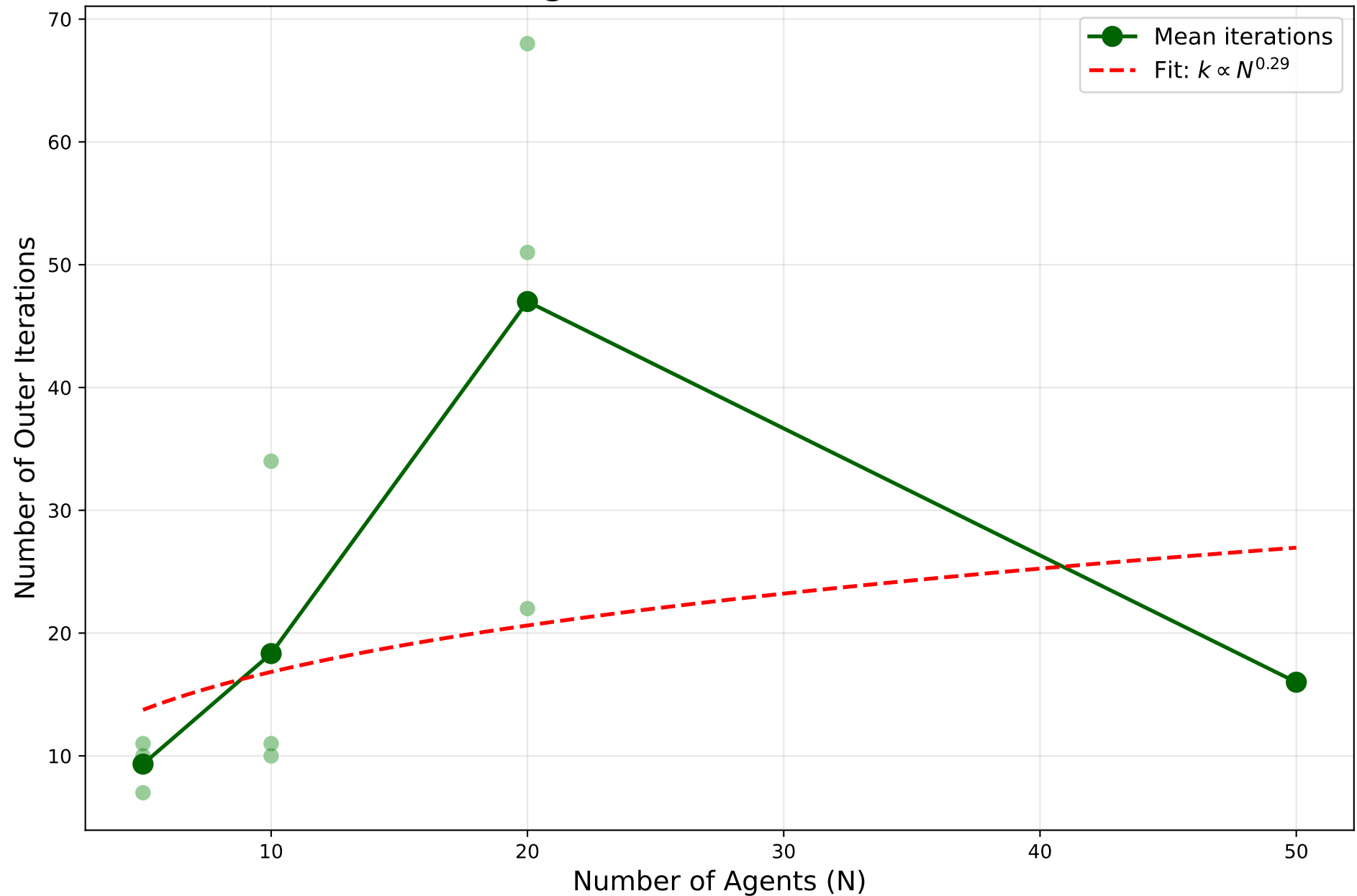
DRPG Convergence: Iterations vs Problem Size
