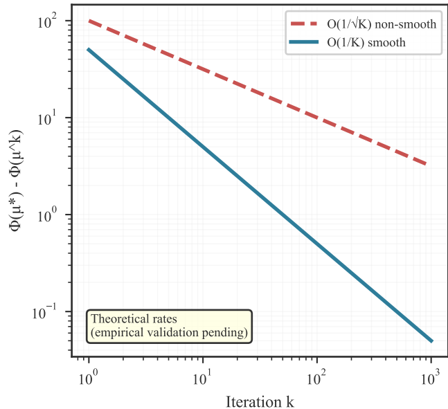
(B) PRDA Dual Gap Decay
