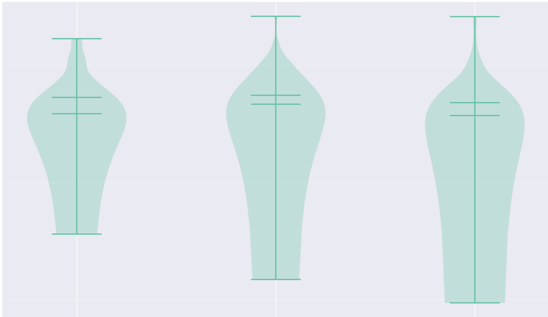
Error Distribution by Uncertainty Set ( \epsilon=1.0\text{e-}06 )
