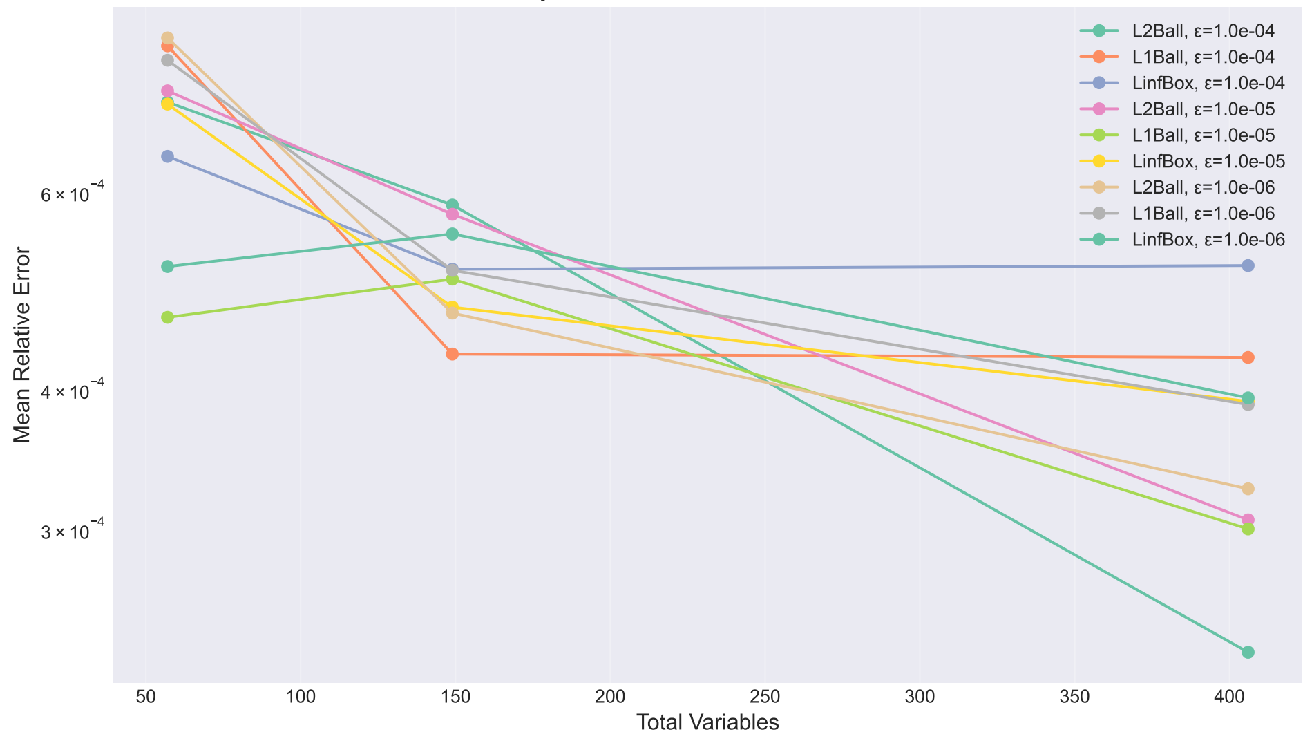
Envelope Theorem Error vs Problem Size
