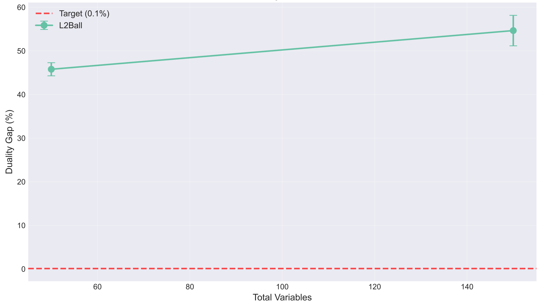
Primal-Dual Gap vs Problem Size
