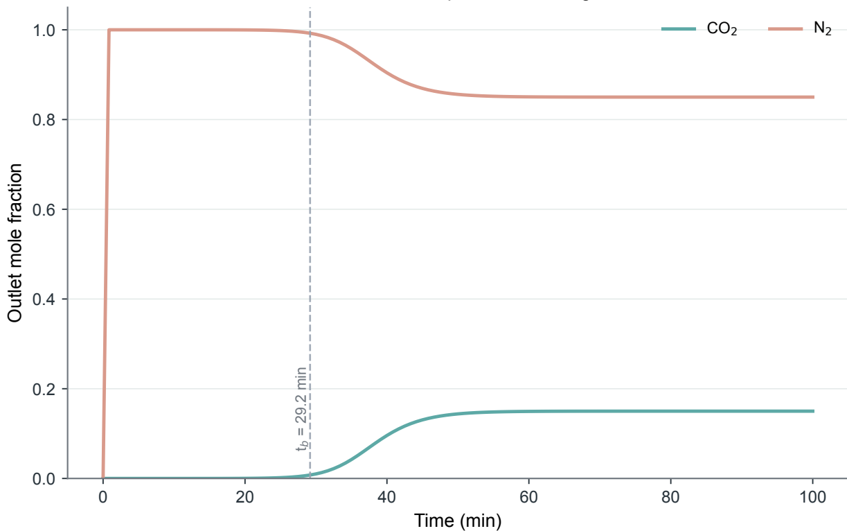
Fixed-bed adsorption breakthrough
