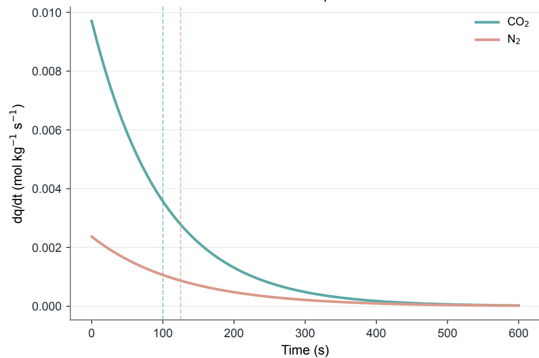
LDF rate response
