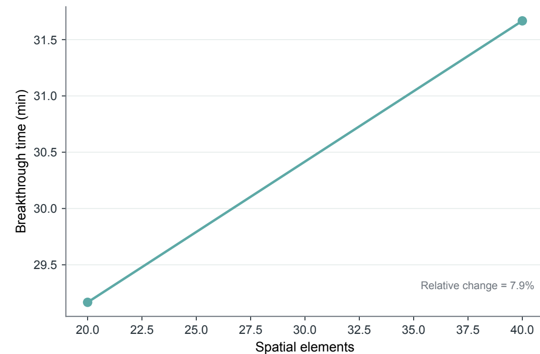
Fixed-bed mesh check
