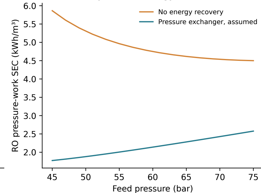
f Hydraulic energy scenarios
