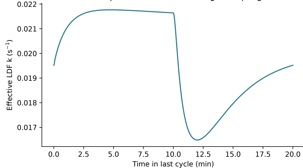
f Temperature + diffusion-length coupling
