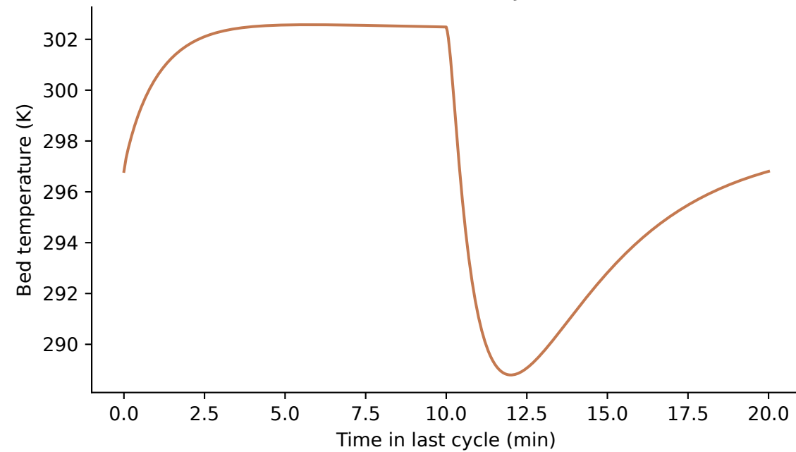
f Temperature + diffusion-length coupling
