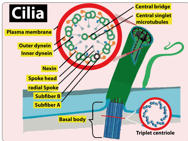
Cilium / flagellum = 9+2 AXONEME (9 outer doublets + 2 central)
