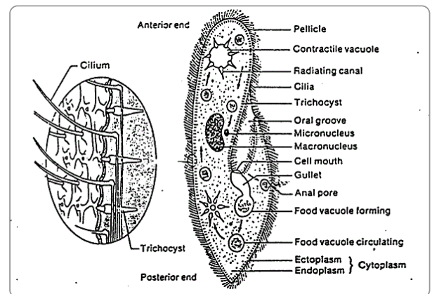
CILIOPHORA - Paramecium external + internal (2 nuclei, cilia, oral groove)
