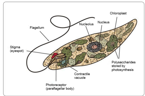
MASTIGOPHORA - Euglena (flagellum + eyespot + chloroplast = mixotroph)
