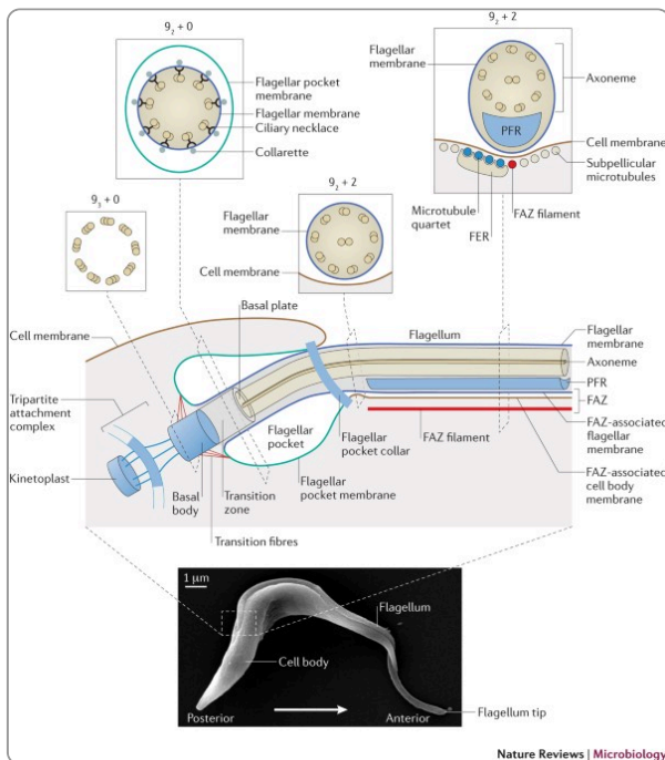
Mastigophora - Trypanosoma (1 flagellum + undulating membrane, parasite)
