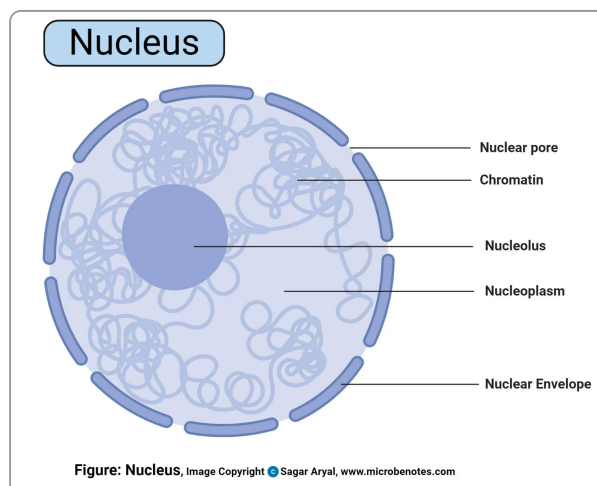
Nucleus: envelope + pores + nucleolus + chromatin (draw & label)
