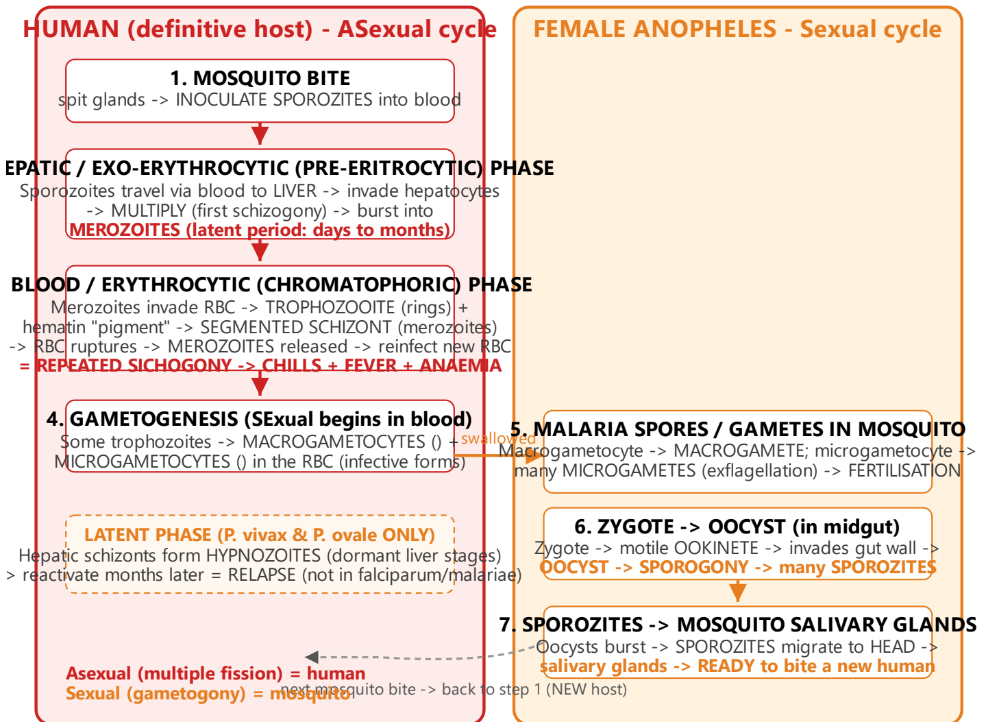
Fig 3: Plasmodium complete life cycle - 7 numbered stages spanning HUMAN (asexual: hepatic + blood schizogony) and FEMALE ANOPHELES (sexual: gametogony + sporogony), plus the vivax/ovale hypnozoite relapse box
