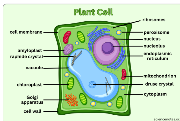
Plant cell = animal + cell wall + chloroplast + big vacuole, NO centriole
