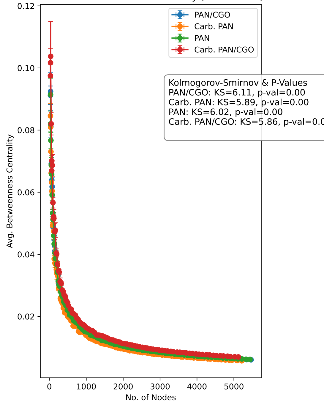
Nodes vs Betweenness Centrality (Actual Data)
