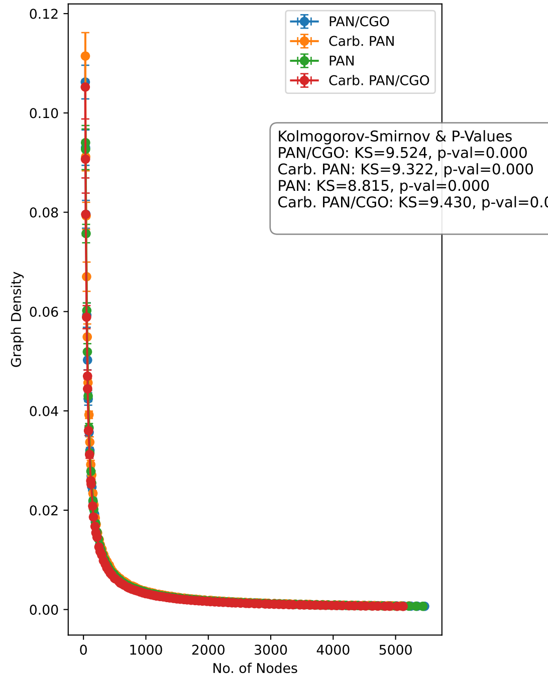
Nodes vs Graph Density (Actual Data)
