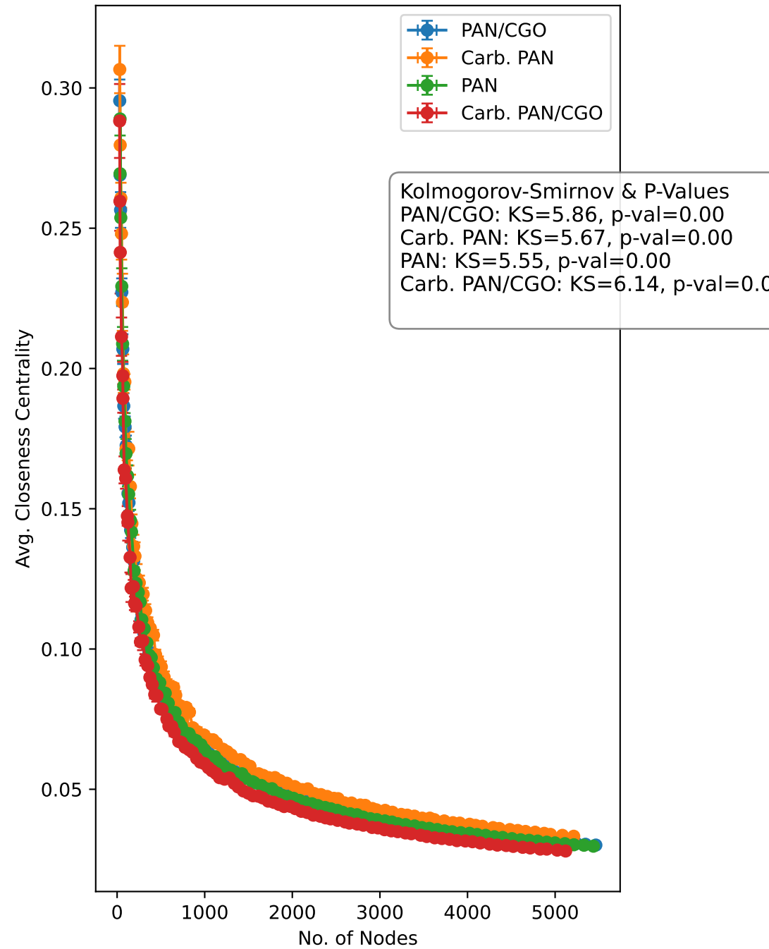
Nodes vs Closeness Centrality (Actual Data)
