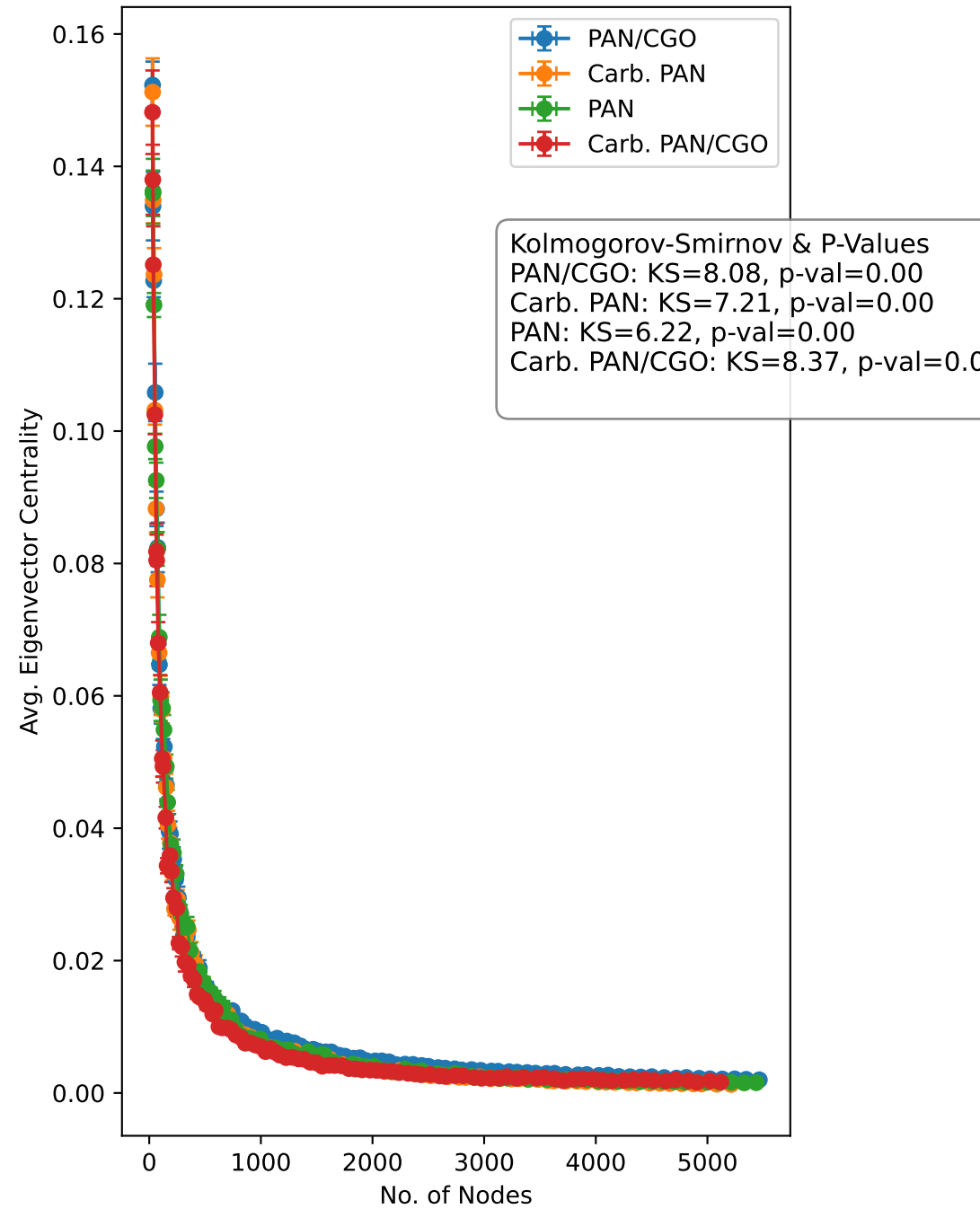
Nodes vs Eigenvector Centrality (Actual Data)
