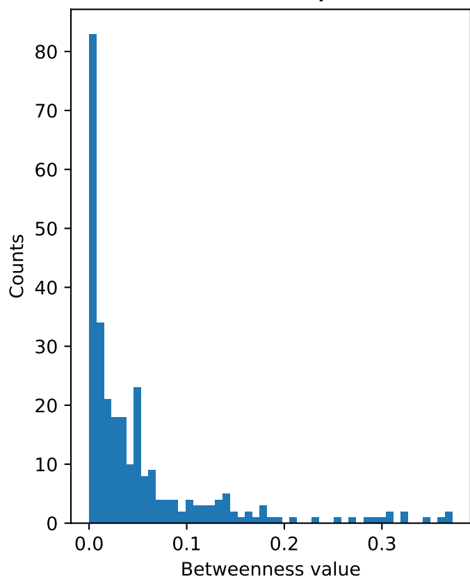
Betweenness Centrality: \sigma=0.074
