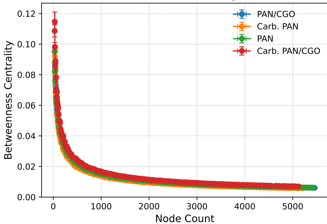
Gamma Fit: y = a \cdot \frac{x^{\alpha-1}}{\Gamma(\alpha)} \cdot \frac{\exp(-\frac{x}{\theta})}{\Gamma(\alpha)\theta^{\alpha}} Nodes vs Betweenness Centrality
