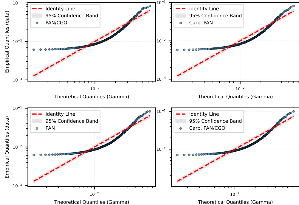
Log Q-Q Plot (Gamma): Betweenness Centrality
