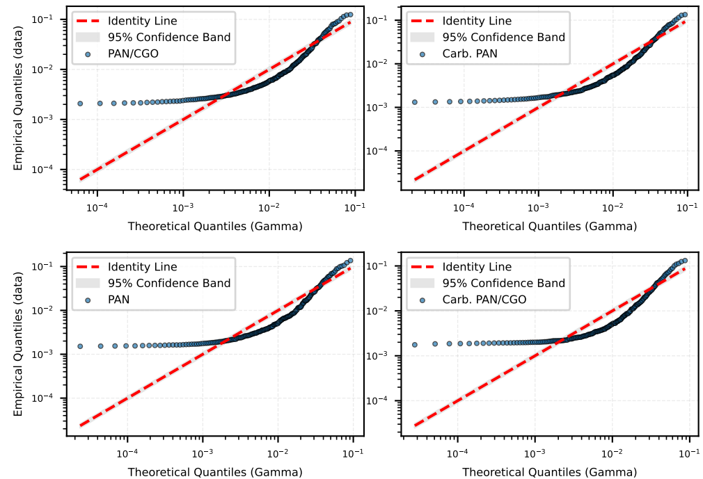
Log Q-Q Plot (Gamma): Eigenvector Centrality
