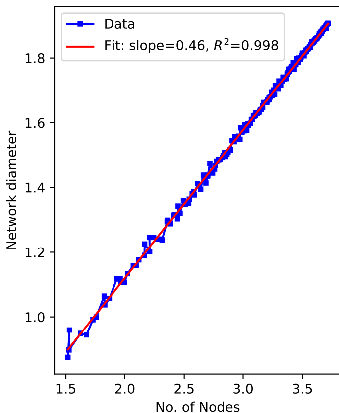
Log-Normal Fit and Plot of Nodes vs Network diameter
