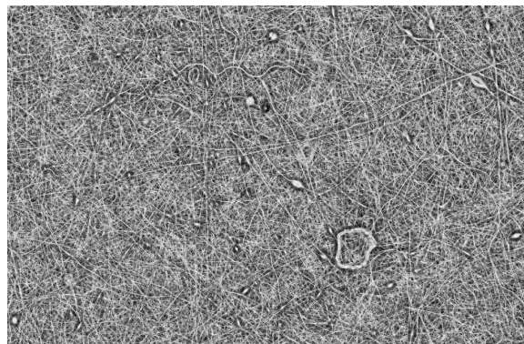
Processed Image
