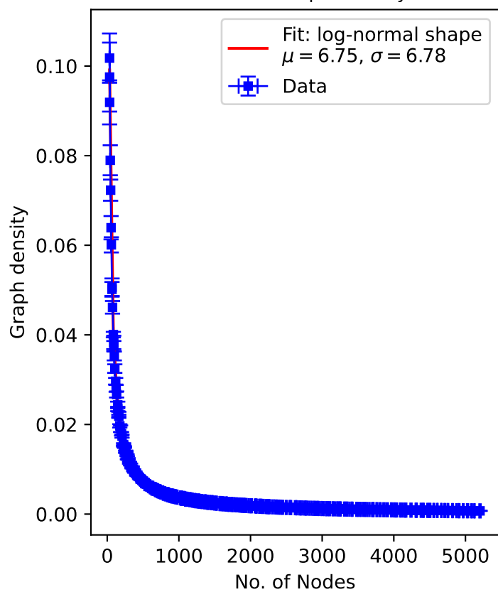
Log-Normal Fit and Plot of Nodes vs Graph density
