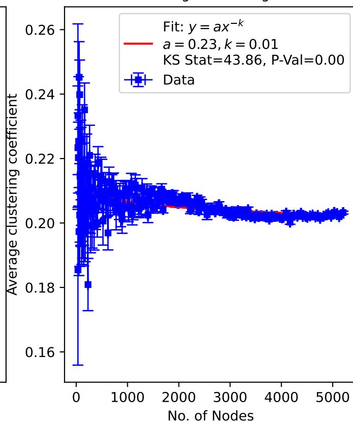
Power Law Fit and Plot of Nodes vs Average clustering coefficient
