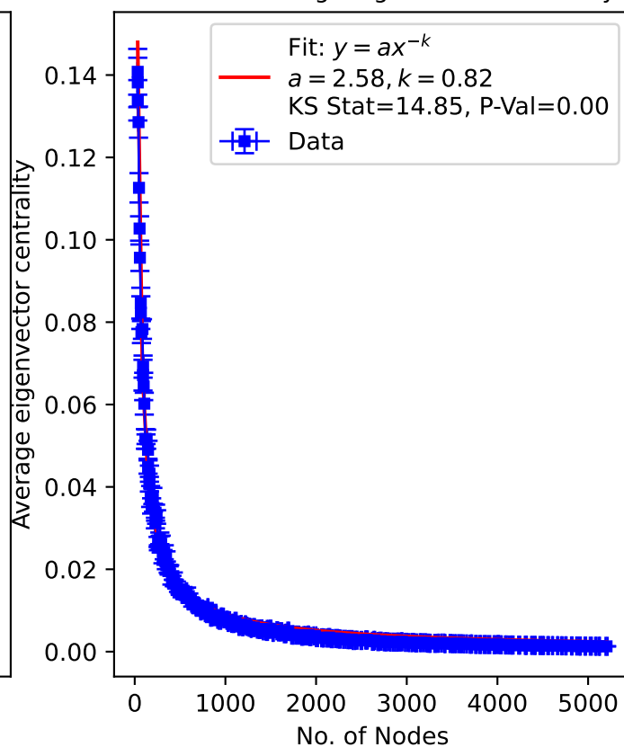
Power Law Fit and Plot of Nodes vs Average eigenvector centrality
