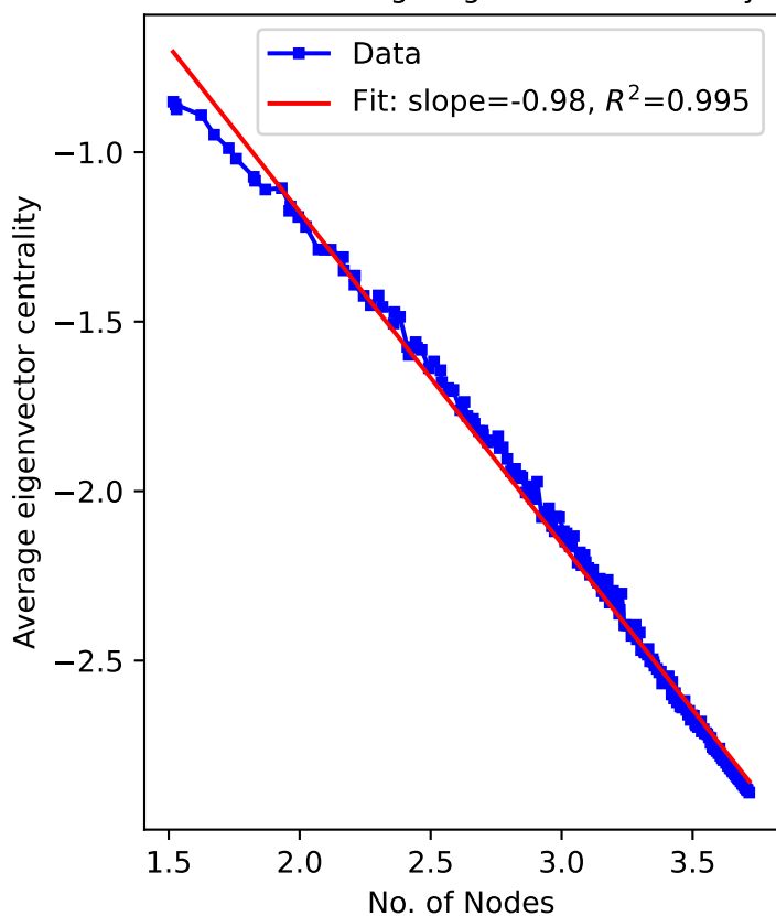
Log-Normal Fit and Plot of Nodes vs Average eigenvector centrality
