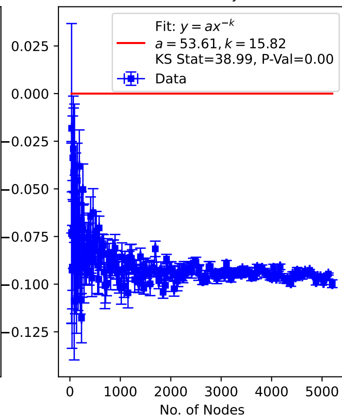
Power Law Fit and Plot of Nodes vs Assortativity coefficient
