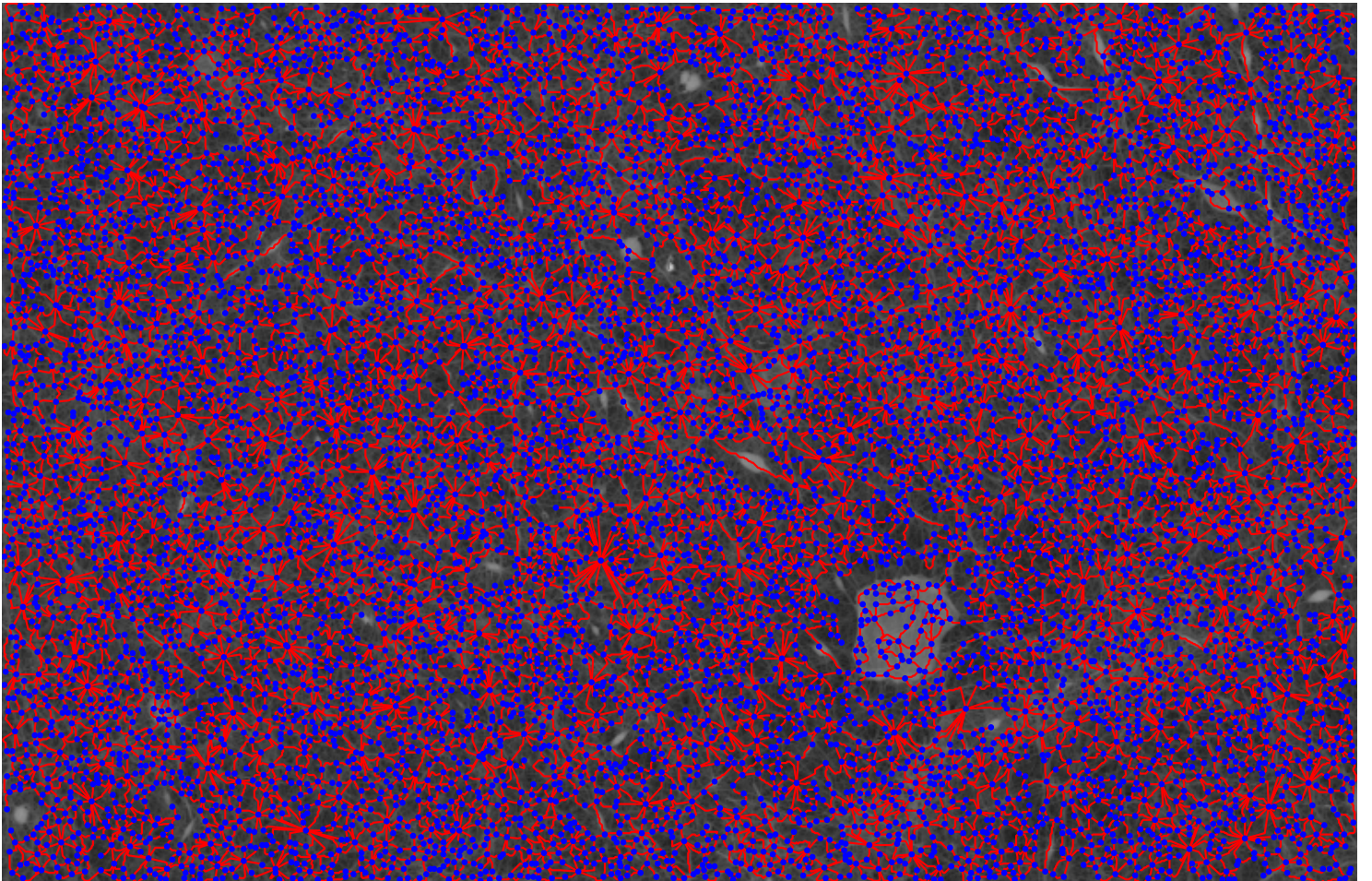
Graph Node Plot
