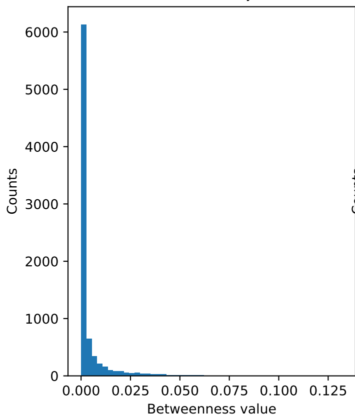
Betweenness Centrality: \sigma=0.012
