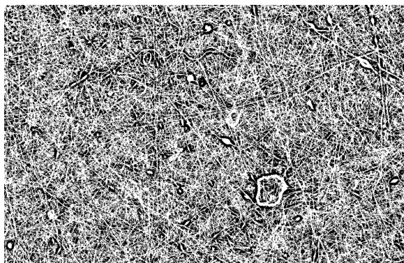
Binary Image
