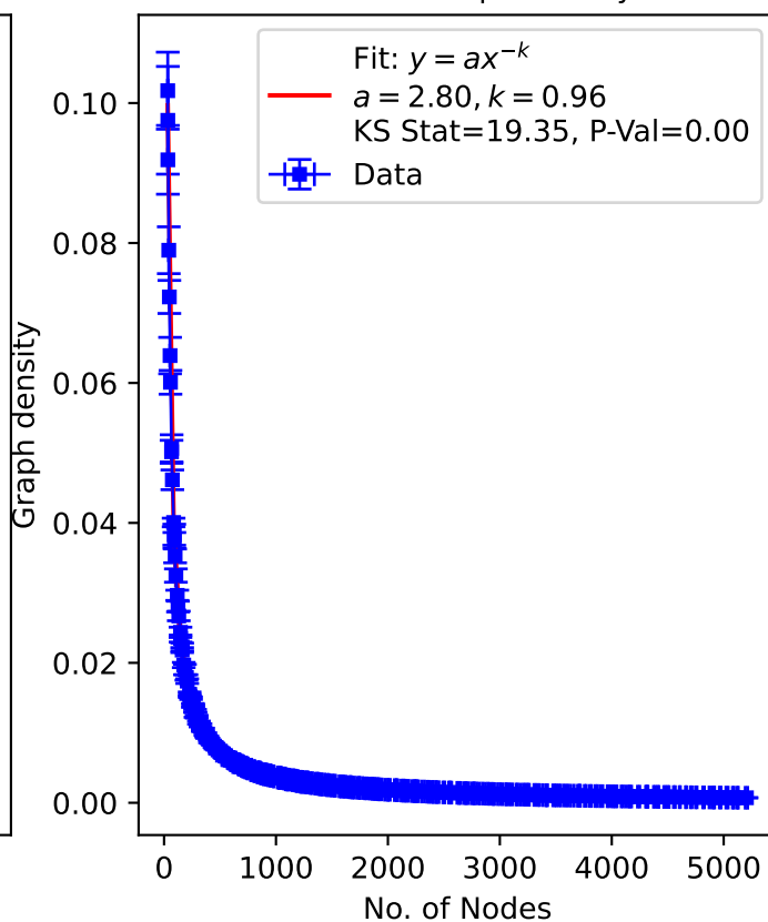
Power Law Fit and Plot of Nodes vs Graph density
