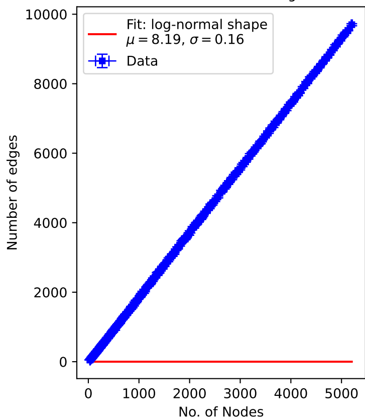
Log-Normal Fit and Plot of Nodes vs Number of edges
