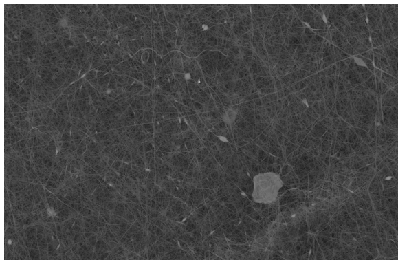
Original Image
