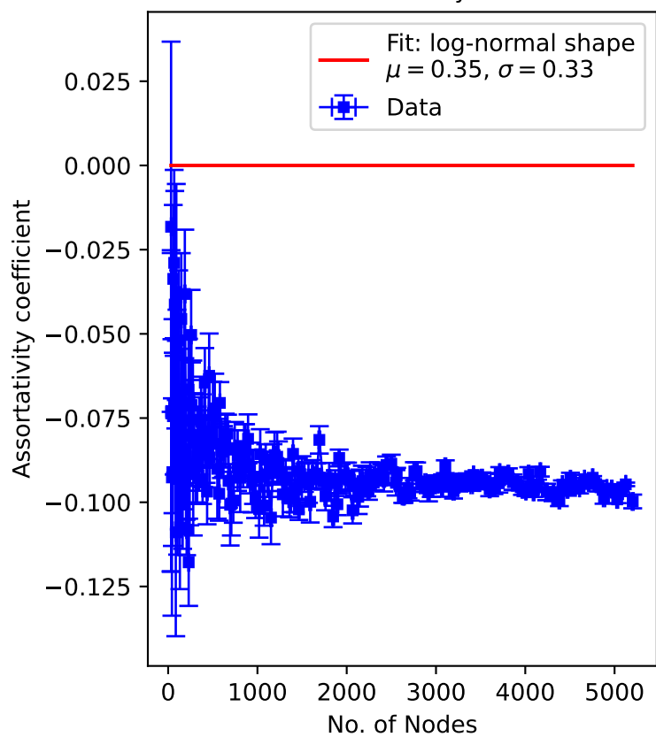
Log-Normal Fit and Plot of Nodes vs Assortativity coefficient
