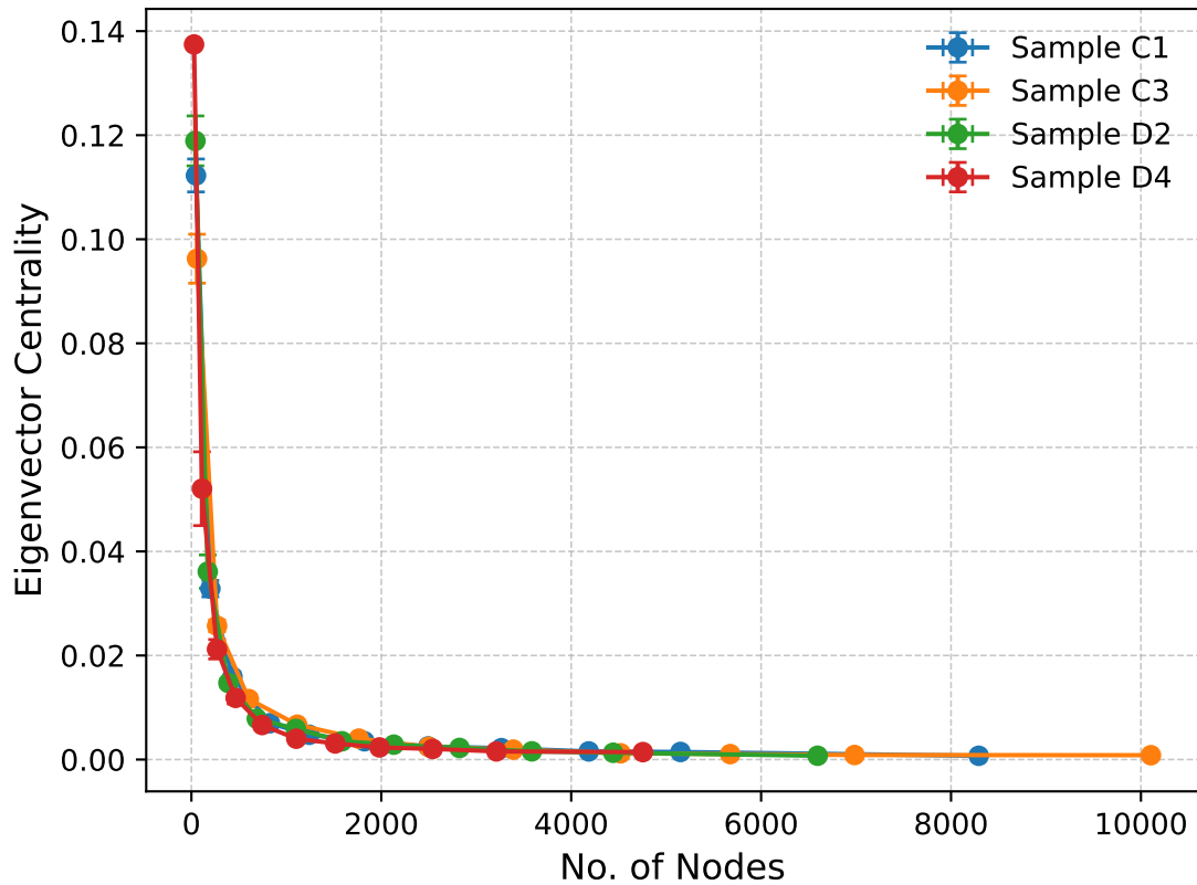
Nodes vs Eigenvector Centrality (Actual Data)
