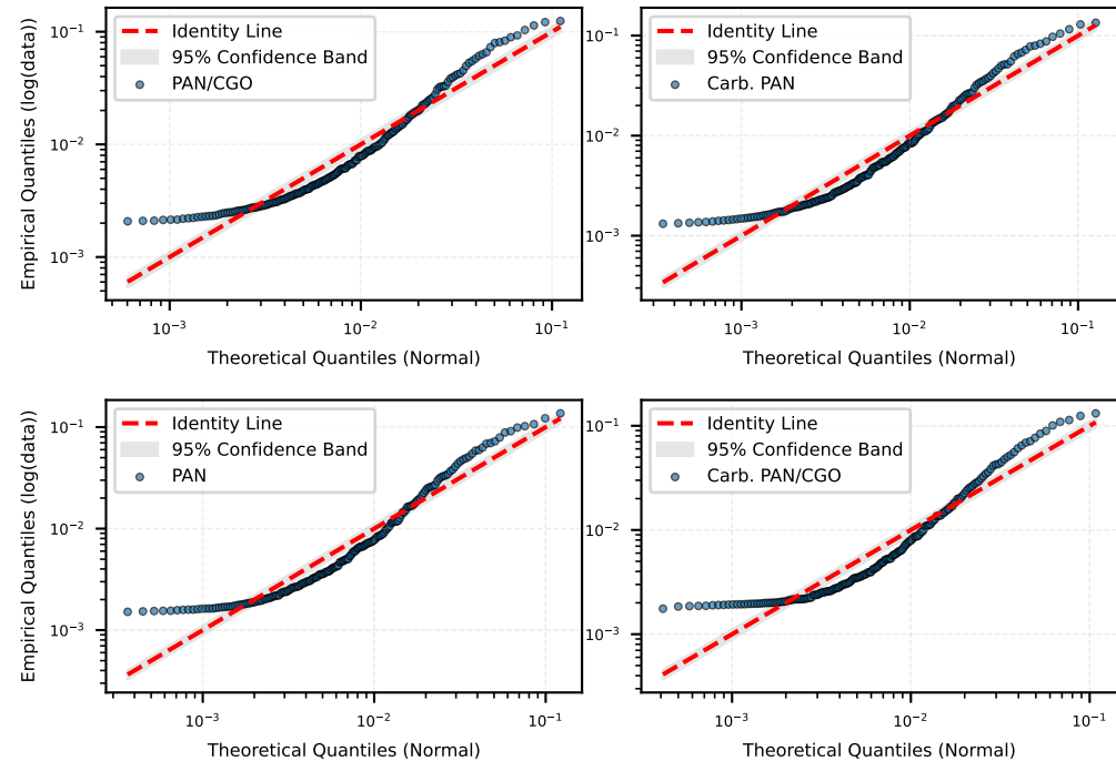
Log Q-Q Plot (Lognormal): Eigenvector Centrality
