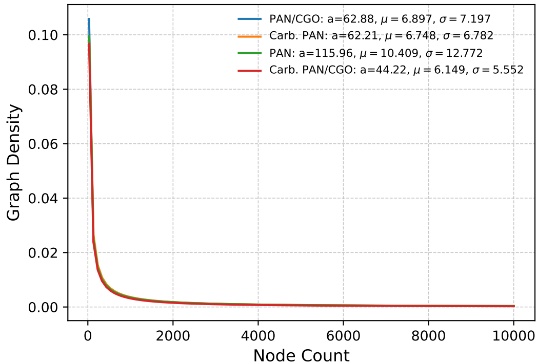
Nodes vs Graph Density
