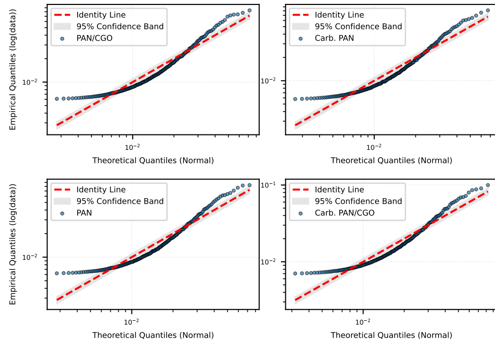
Log Q-Q Plot (Lognormal): Betweenness Centrality
