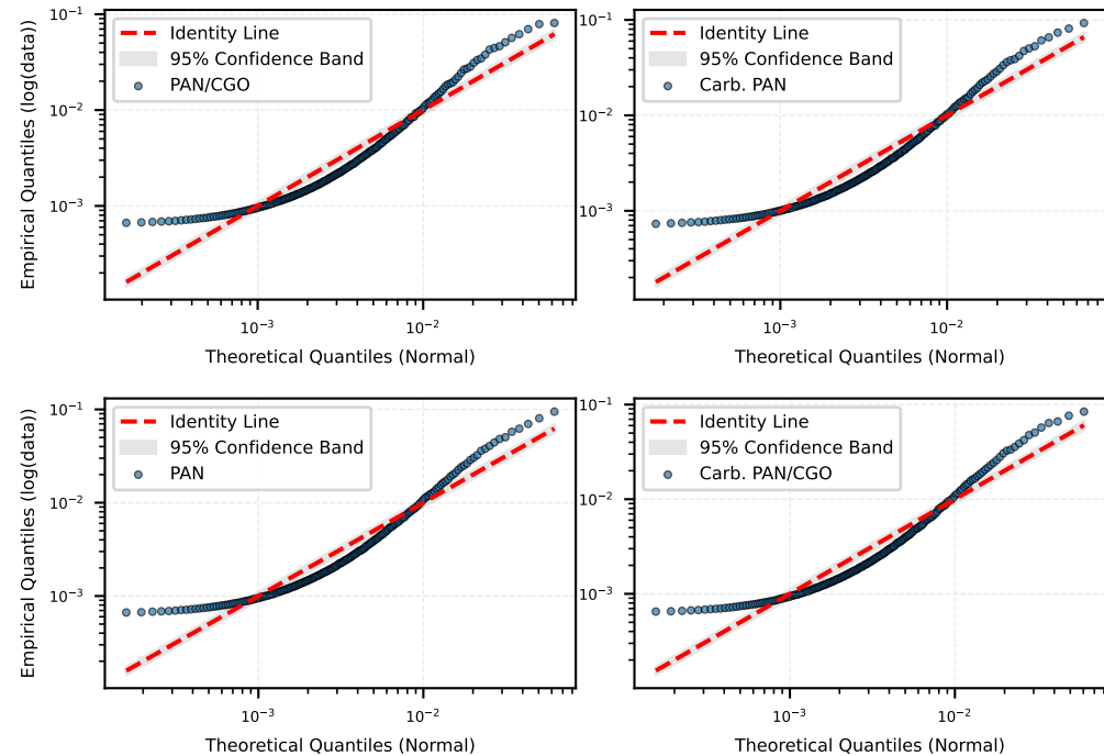
Log Q-Q Plot (Lognormal): Graph Density
