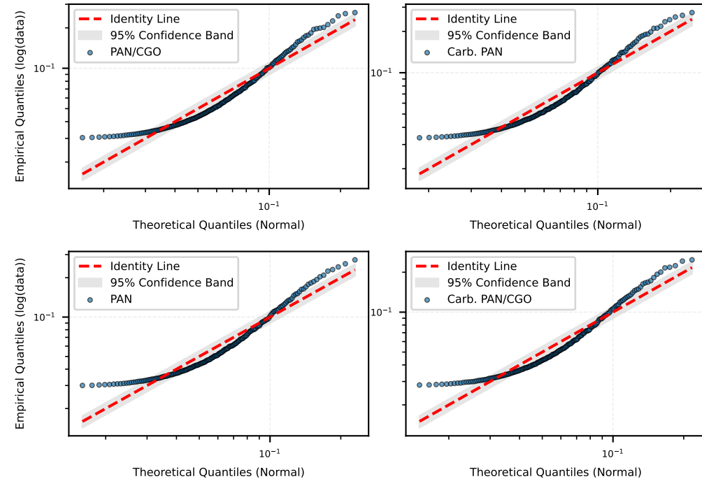
Log Q-Q Plot (Lognormal): Closeness Centrality
