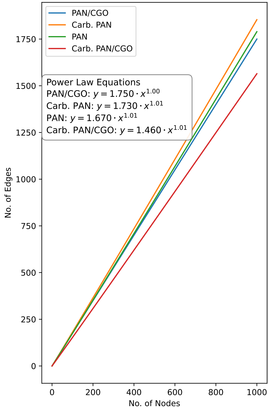
Nodes vs Edges (Power Law Fit)
