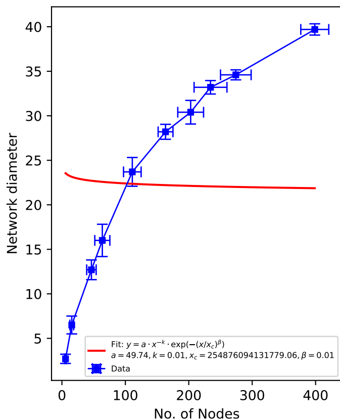
Power Law (w. Exponential Cutoff) Fit Nodes vs Network diameter
