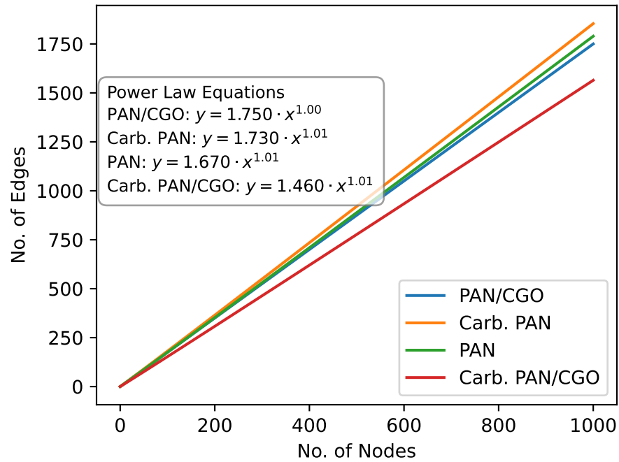
Nodes vs Edges (Power Law Fit)
