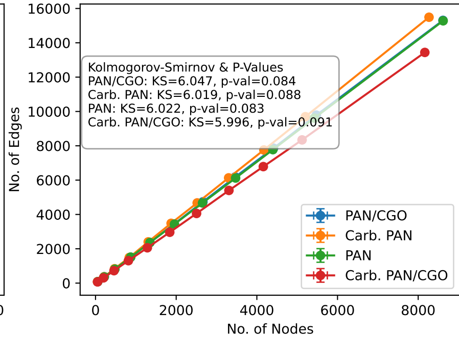
Nodes vs Edges (Actual Data)
