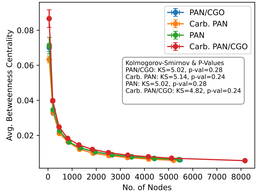
Nodes vs Betweenness Centrality (Actual Data)
