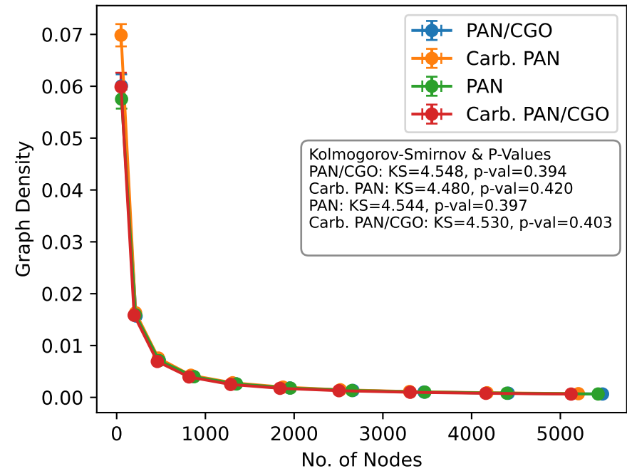
Nodes vs Graph Density (Actual Data)
