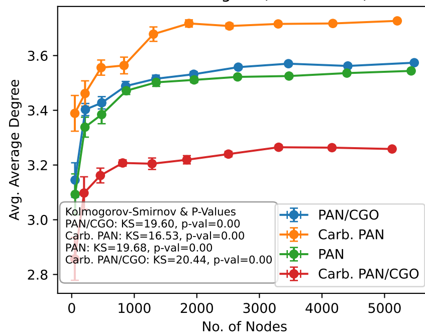
Nodes vs Degree (Actual Data)
