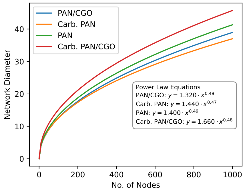
Nodes vs Network Diameter (Power Law Fit)
