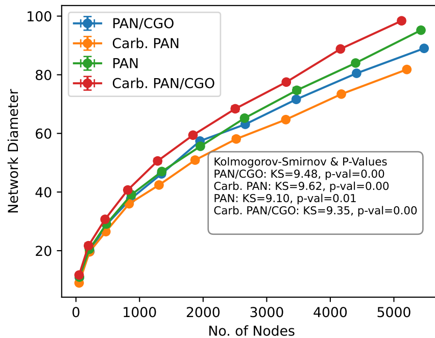
Nodes vs Network Diameter (Actual Data)
