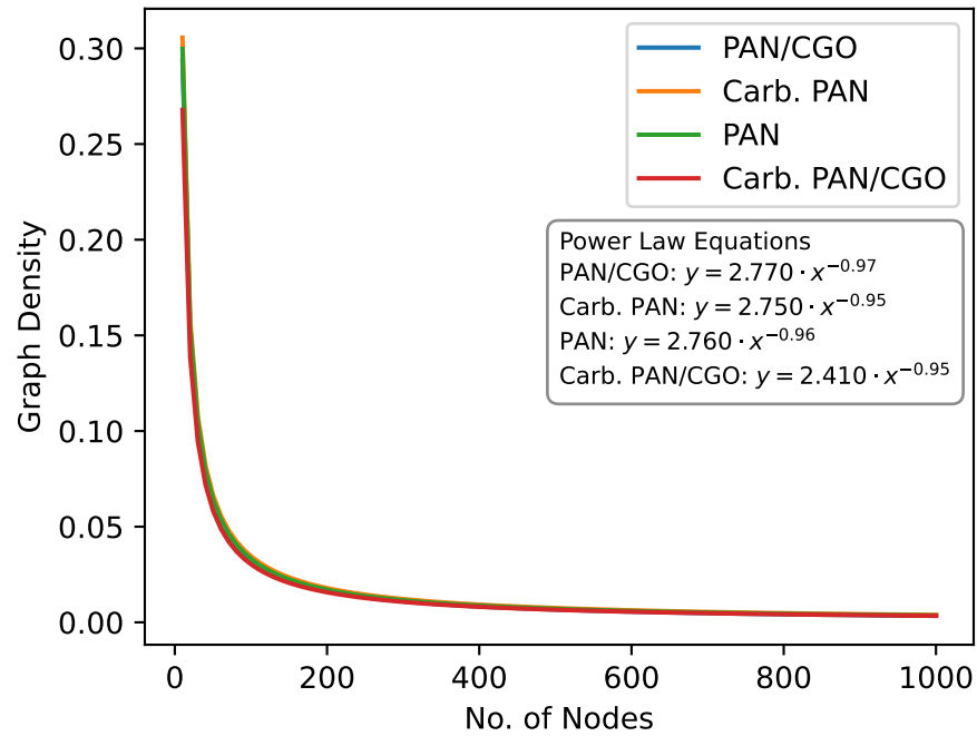
Nodes vs Graph Density (Power Law Fit)
