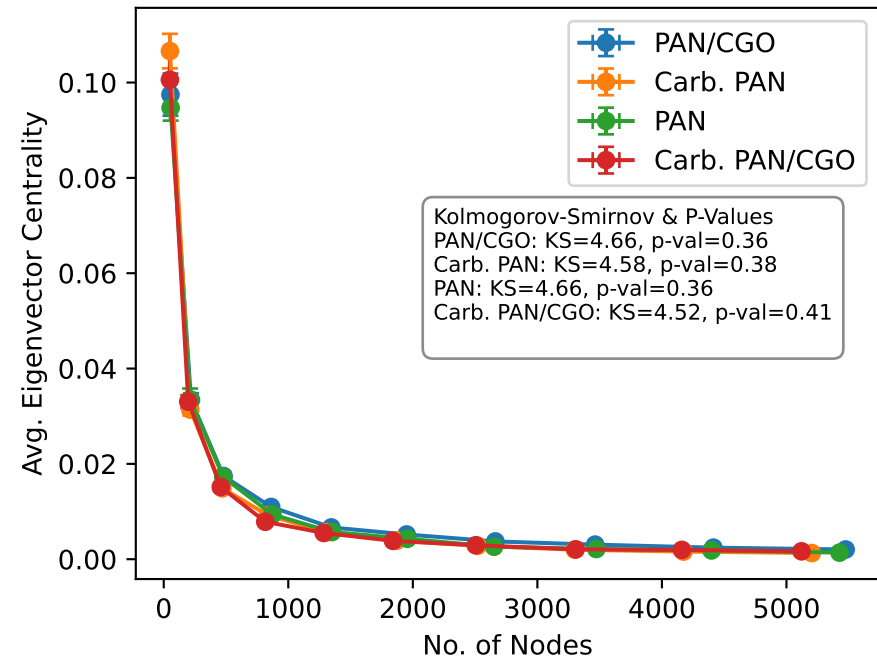
Nodes vs Eigenvector Centrality (Actual Data)
