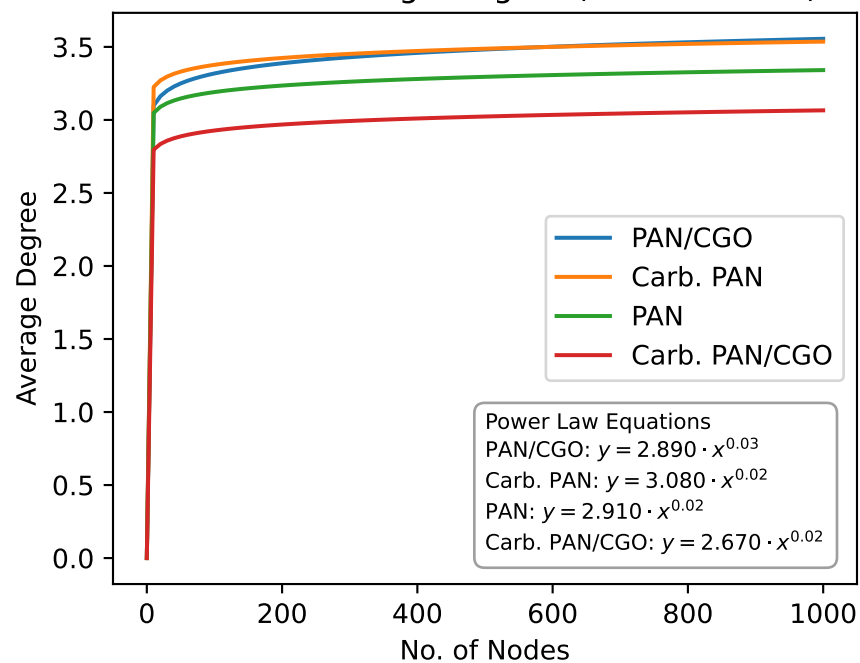
Nodes vs Average Degree (Power Law Fit)
