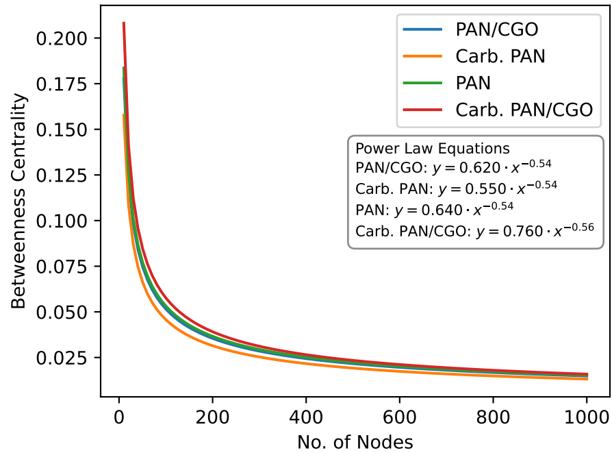
Nodes vs Betweenness Centrality (Power Law Fit)
