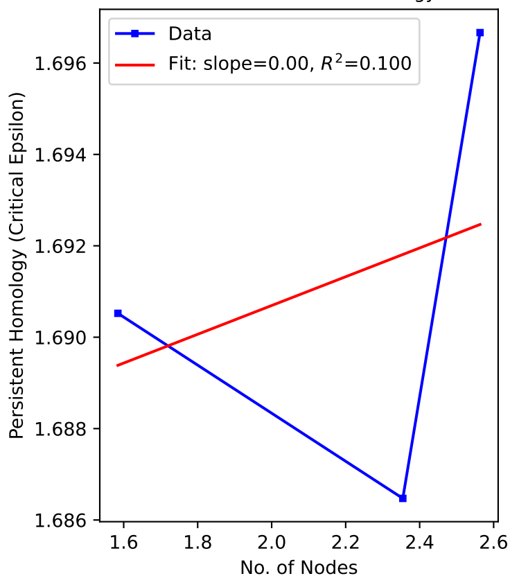
Log-Log Plot of Nodes vs Persistent Homology
