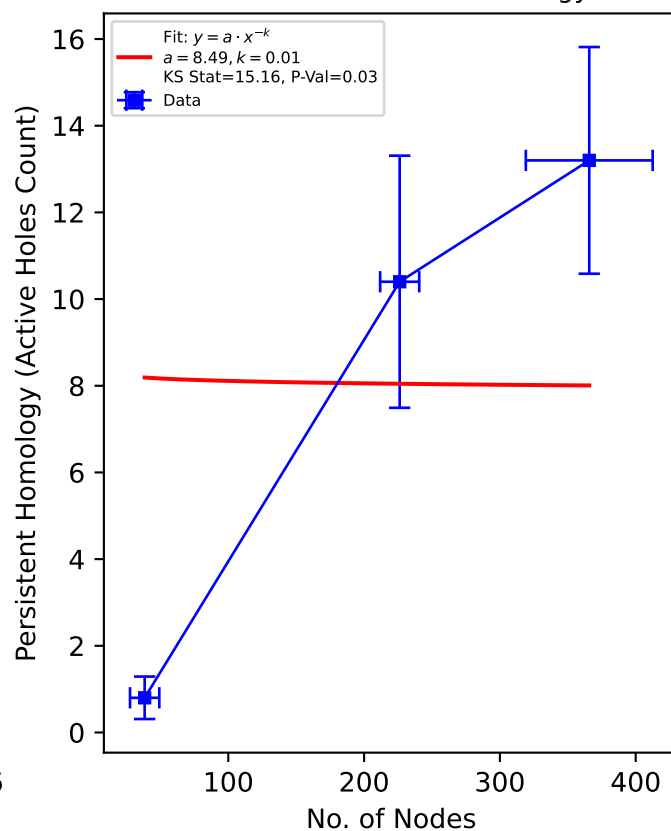
Power Law Fit and Plot of Nodes vs Persistent Homology
