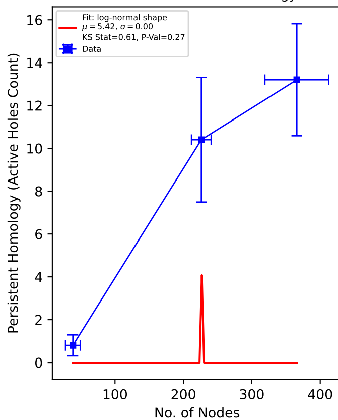
Log-Normal Fit and Plot of Nodes vs Persistent Homology
