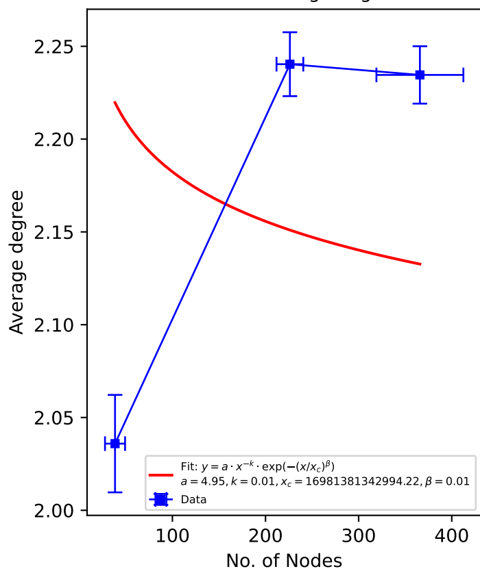
Power Law (w. Exponential Cutoff) Fit Nodes vs Average degree
