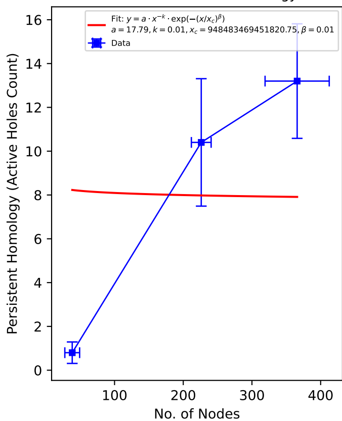
Power Law (w. Exponential Cutoff) Fit Nodes vs Persistent Homology
