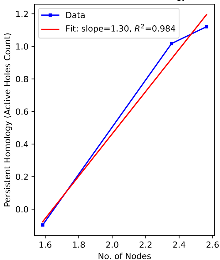
Log-Log Plot of Nodes vs Persistent Homology
