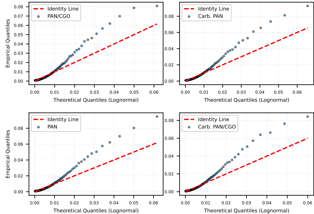
Q-Q Plot: Lognormal Fit for Graph Density
