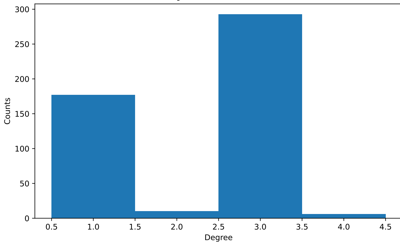
Degree Distribution: \sigma=0.974
