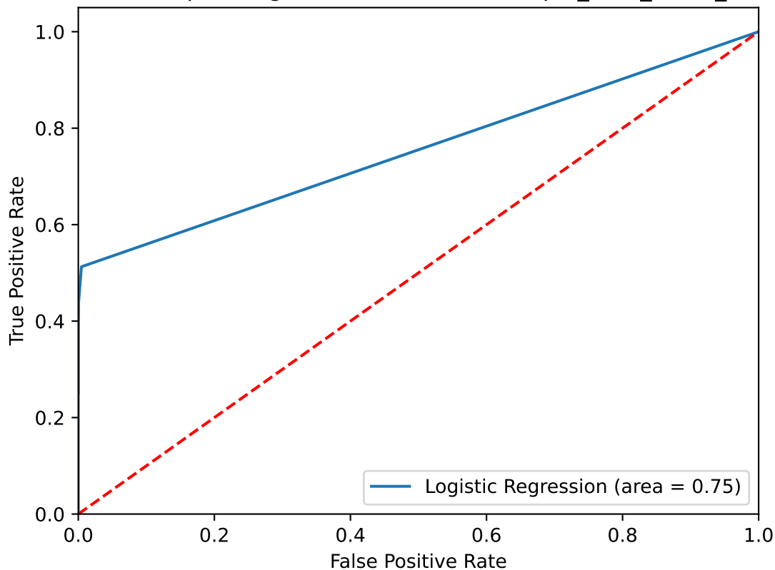
Receiver operating characteristic for Sample_num_reads_300
