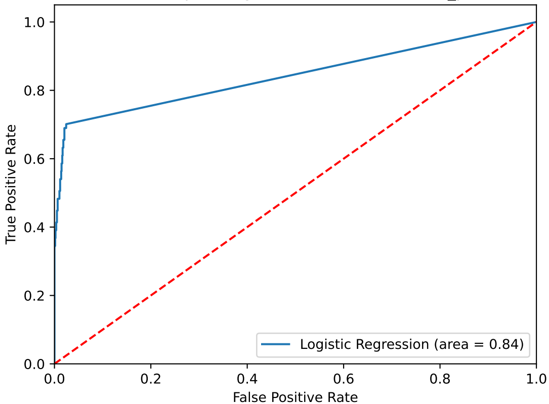
Receiver operating characteristic for bases_perc
