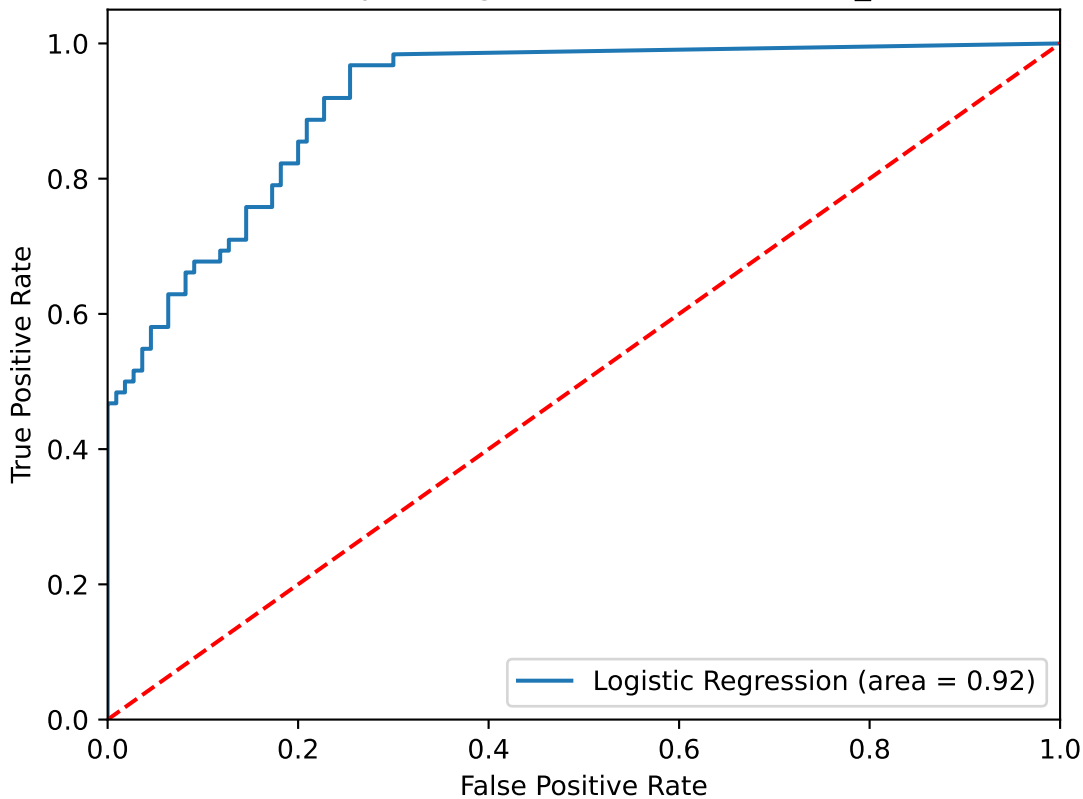
Receiver operating characteristic for AuG_trunc5
