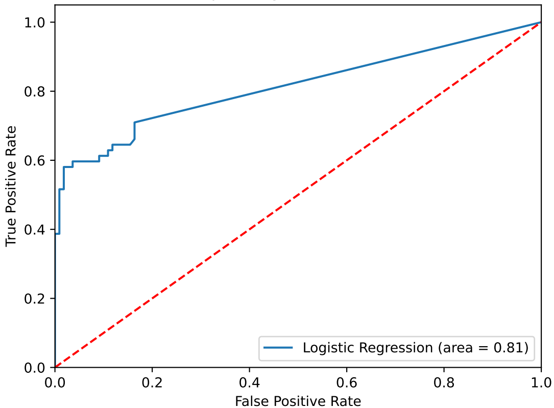
Receiver operating characteristic for Cov3
