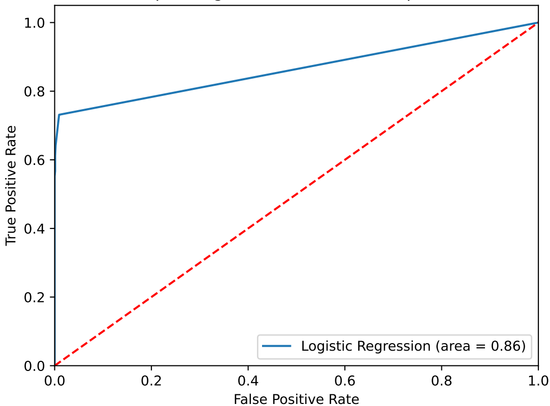
Receiver operating characteristic for sample num reads
