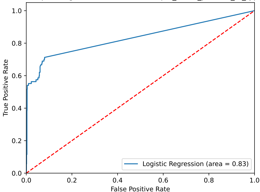
Receiver operating characteristic for Sample_reads_percent_of_type_run
