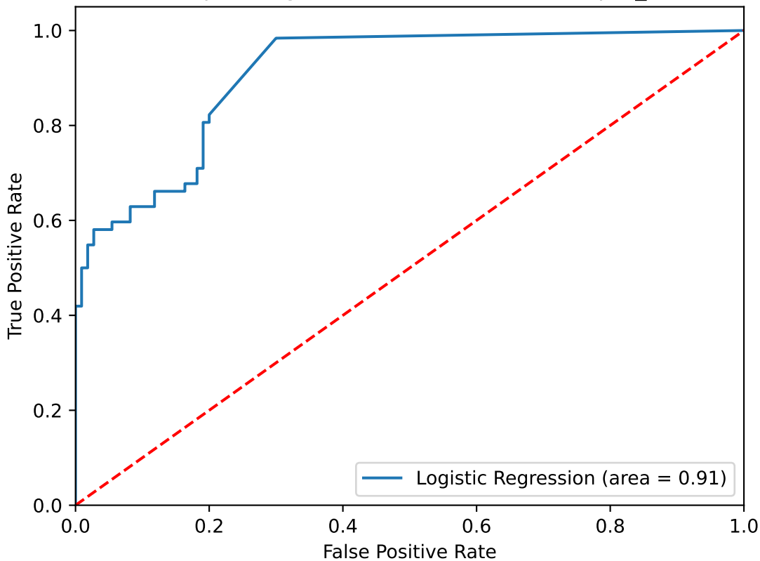
Receiver operating characteristic for meanDepth_trunc10
