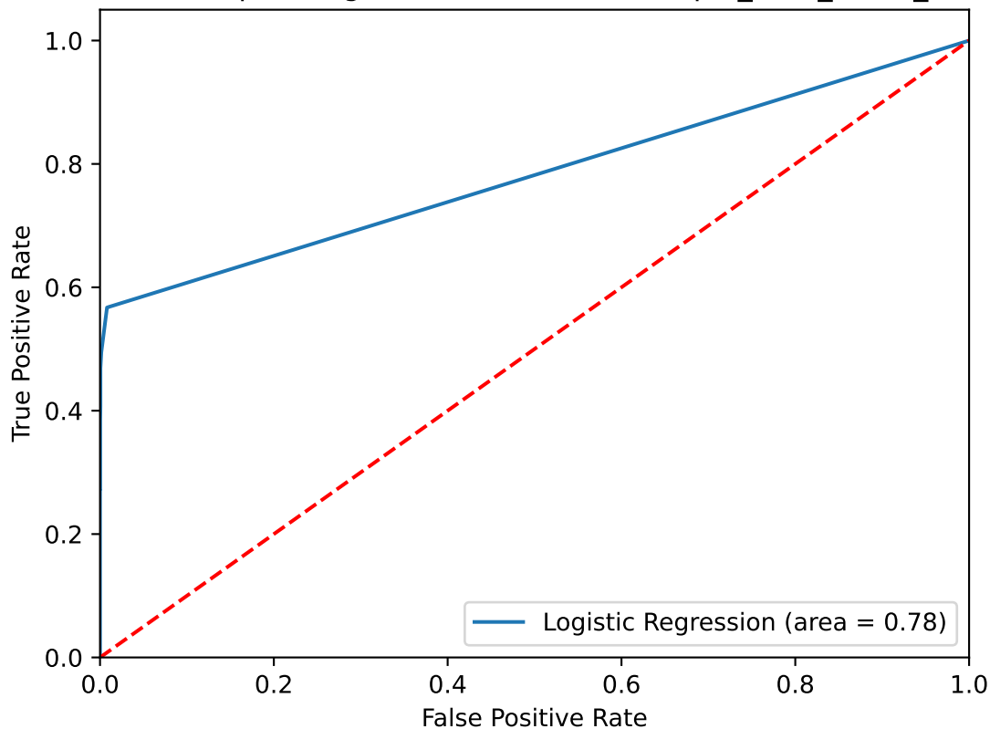
Receiver operating characteristic for Sample_num_reads_200
