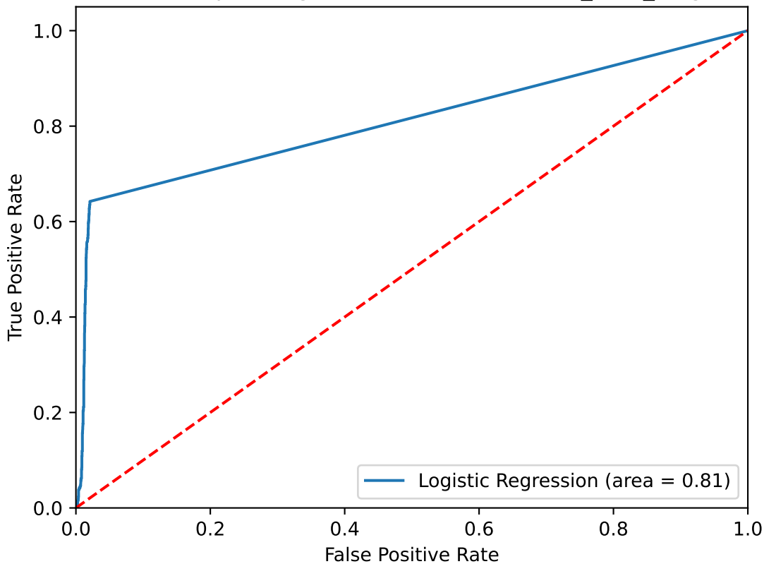
Receiver operating characteristic for mean_read_length
