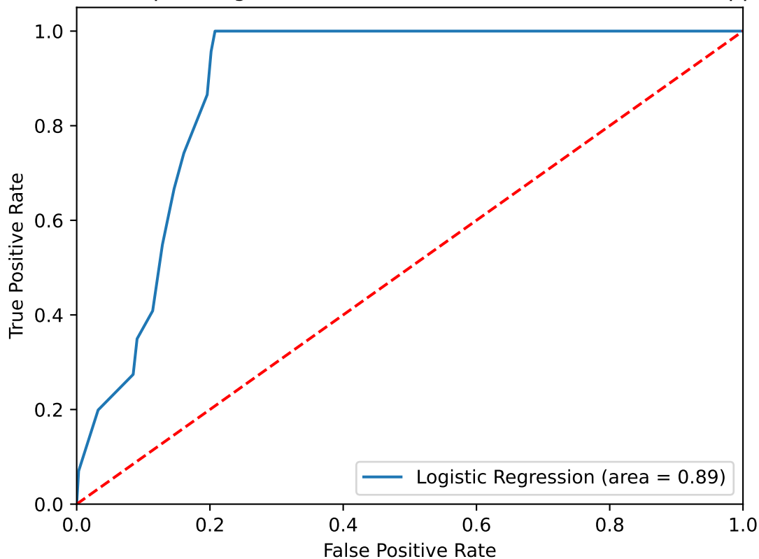
Receiver operating characteristic for total run reads inc unmapped
