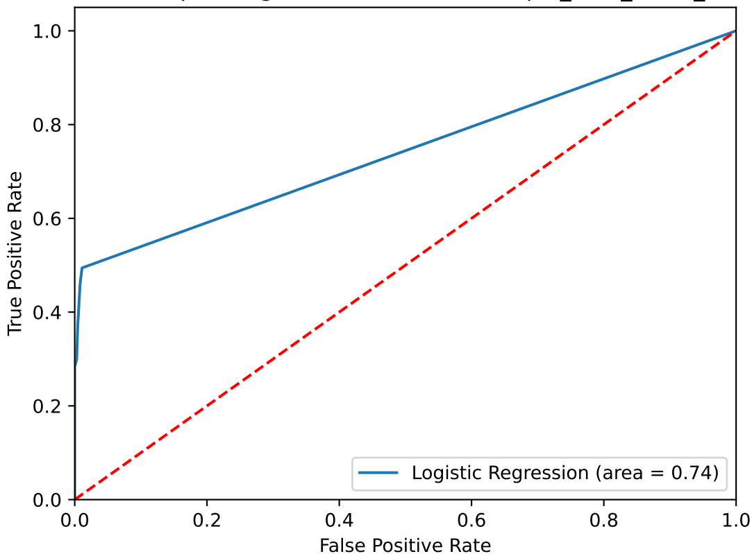
Receiver operating characteristic for Sample_num_reads_400
