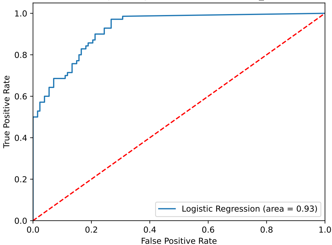
Receiver operating characteristic for AuG_trunc10
