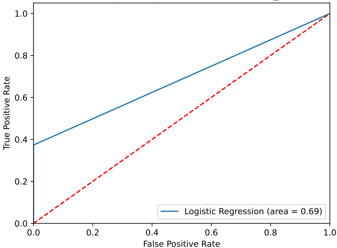
Receiver operating characteristic for Cov5_perc
