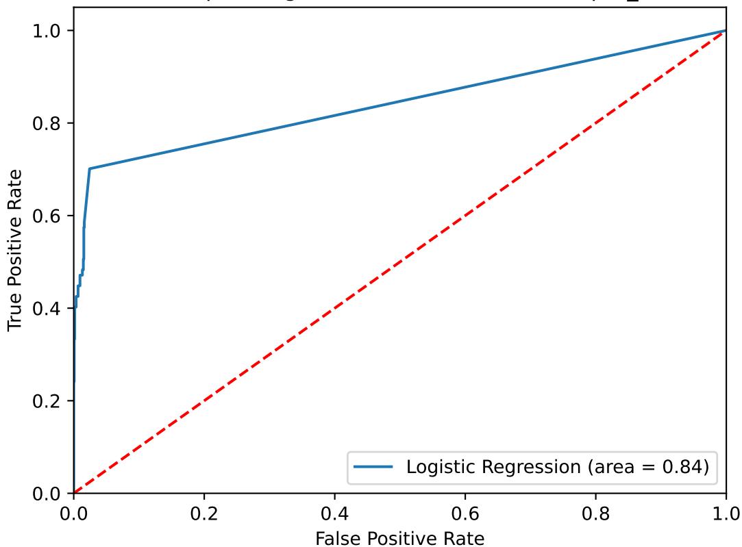
Receiver operating characteristic for meanDepth_trunc5
