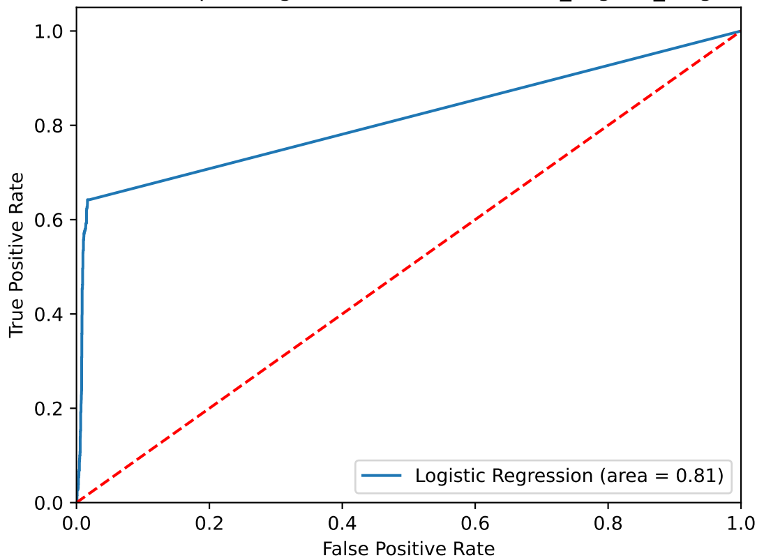
Receiver operating characteristic for mean_aligned_length
