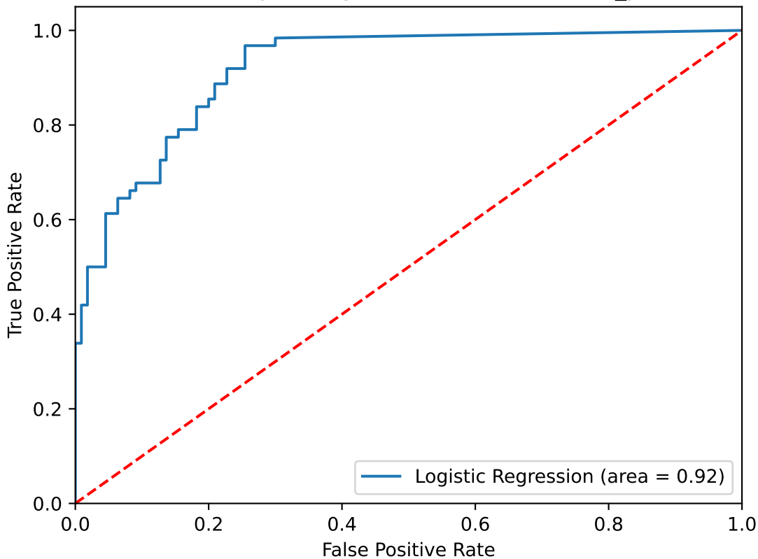
Receiver operating characteristic for Cov1_perc
