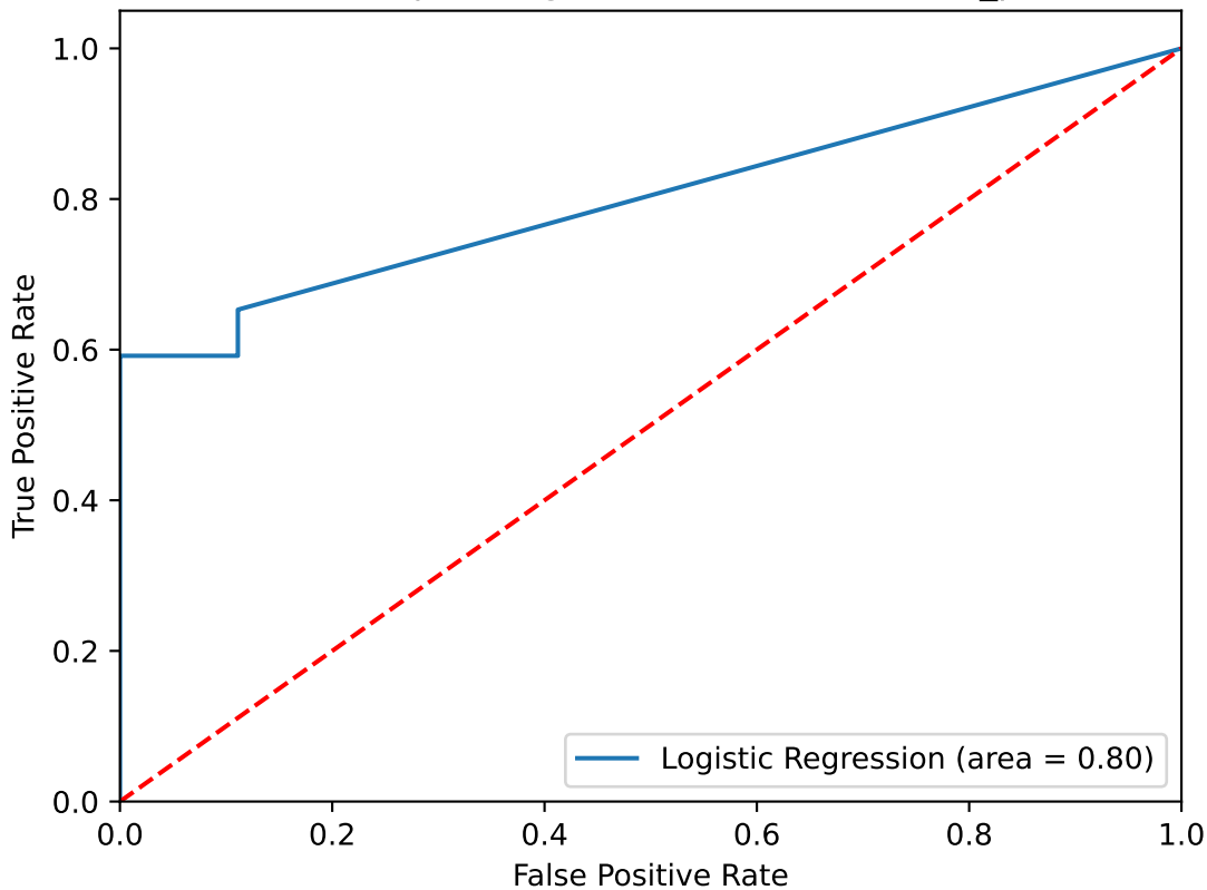
Receiver operating characteristic for Cov3_perc
