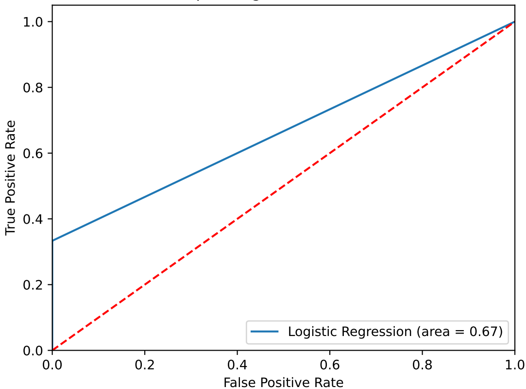
Receiver operating characteristic for Cov10
