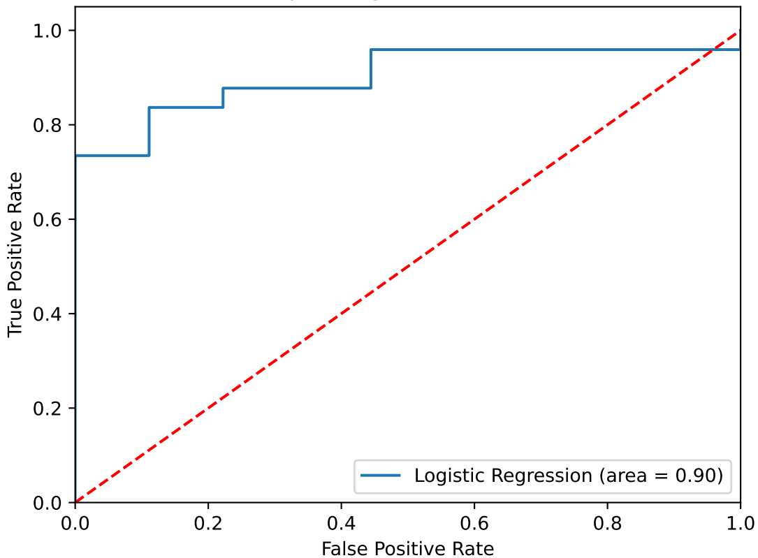
Receiver operating characteristic for Cov1
