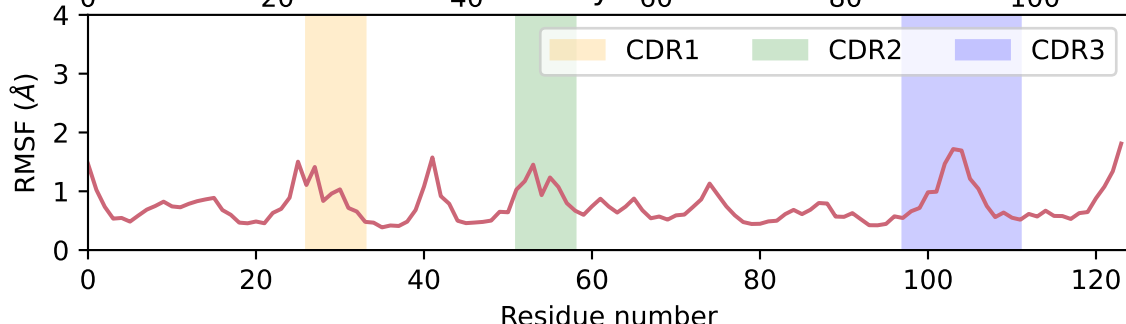
Heavy chain
