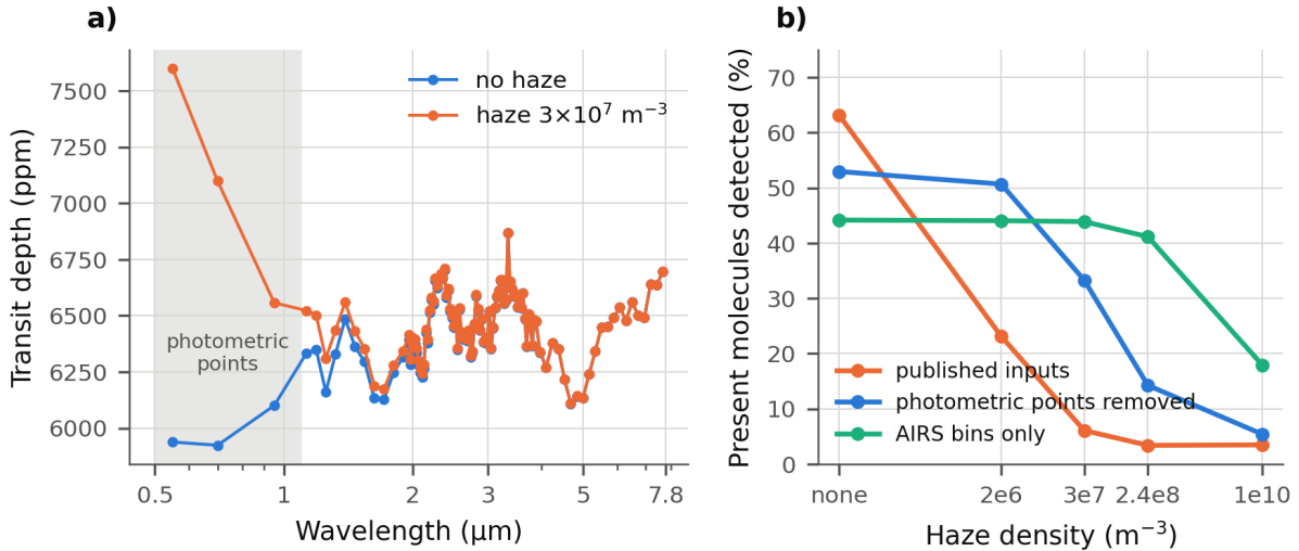
Figure 3. (a) A clear-atmosphere test planet with CH 4 above 10^{-4} at Tier-3 binning, without and with haze at 3 \times 10^7 m -3 (noise-free); shading marks the three photometric points. (b) Detection rate, the share of planets containing a molecule for which it was reported, against haze density for the published input, the input without the
