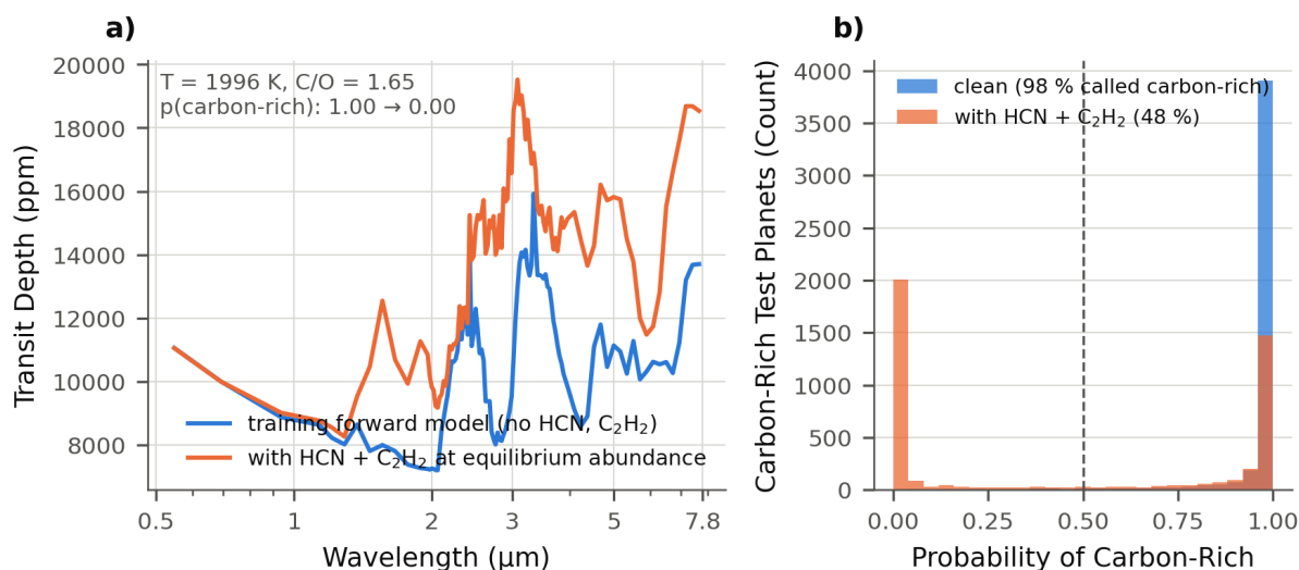
Figure 2. The omitted species. (a) A carbon-rich test planet at the Ariel Tier-3 binning, rendered by the training forward model (blue) and with HCN and \text{C}_2\text{H}_2 added at their equilibrium abundances (orange); the planet shown has the median effect among hot carbon-rich planets. The clean-trained screen's probability of "carbon-rich" for this planet falls from 1.00 to 0.00. (b) The same probability for all 4,508 carbon-rich test planets, clean (blue) and with the two species present (orange): the share called carbon-rich falls from 98 % to 48 %.
