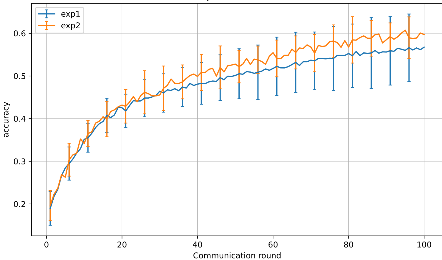
RQ5 client accuracy: mean and standard deviation
