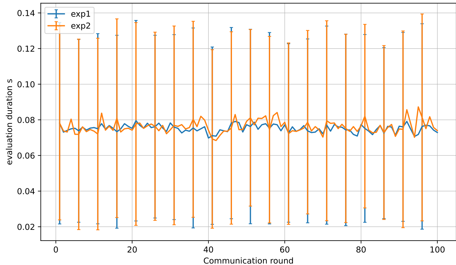
RQ5 client evaluation duration s: mean and standard deviation
