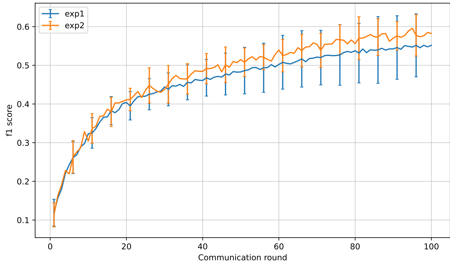
RQ5 client f1 score: mean and standard deviation
