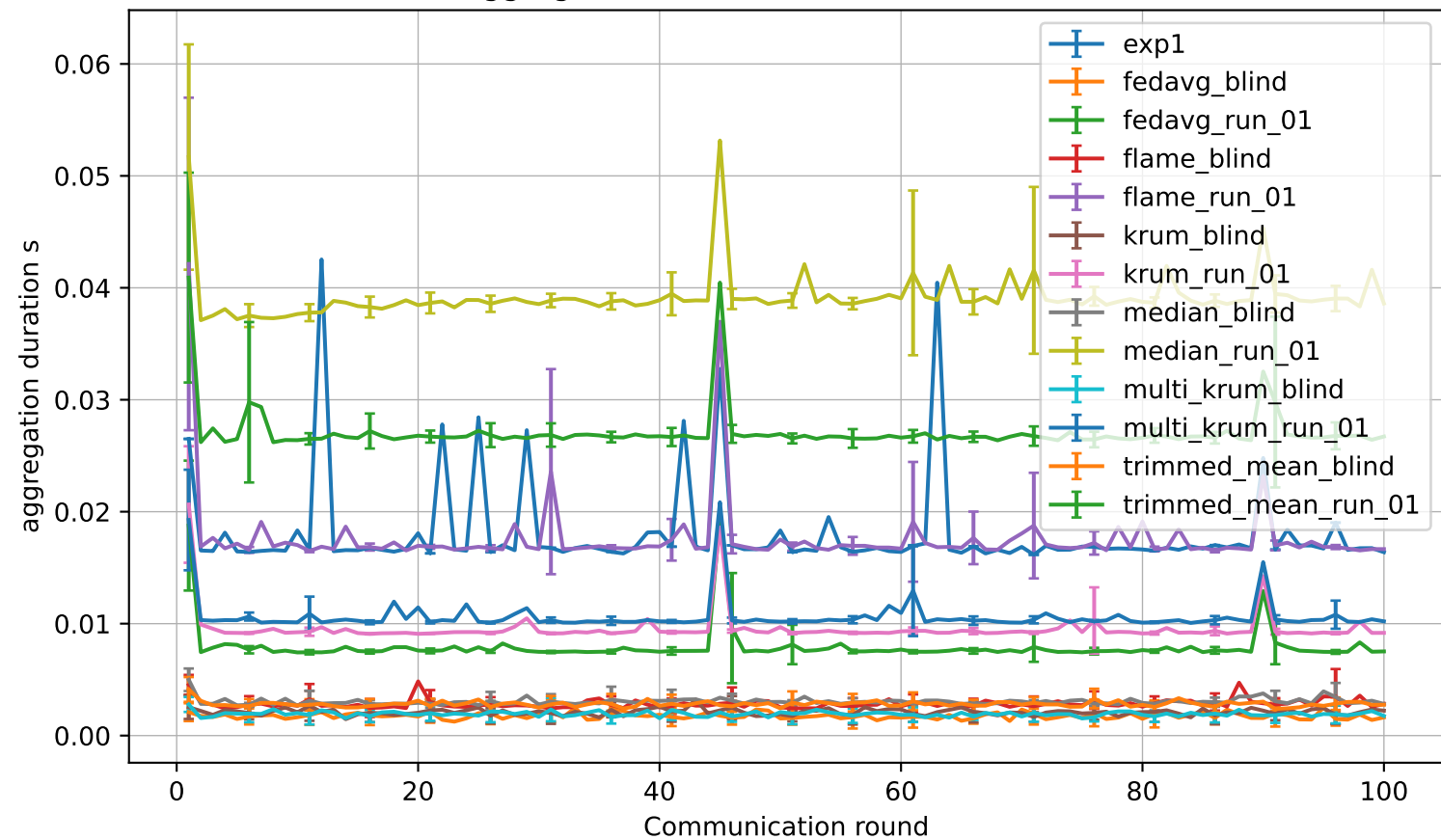
RQ5 server aggregation duration s: mean and standard deviation
