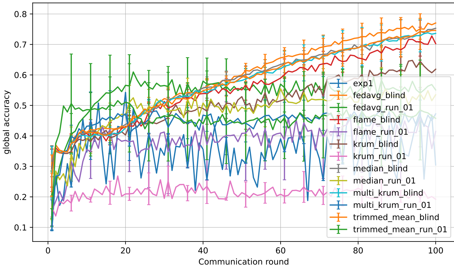
RQ5 server global accuracy: mean and standard deviation
