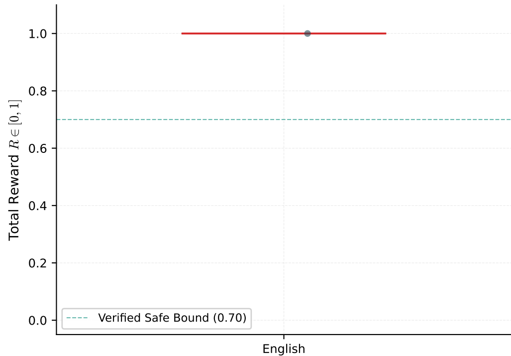
(b) ReST-RL Deliberative Reward Distribution R
